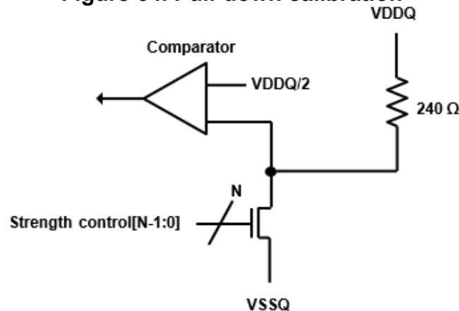
Figure 64. Pull-down calibration
