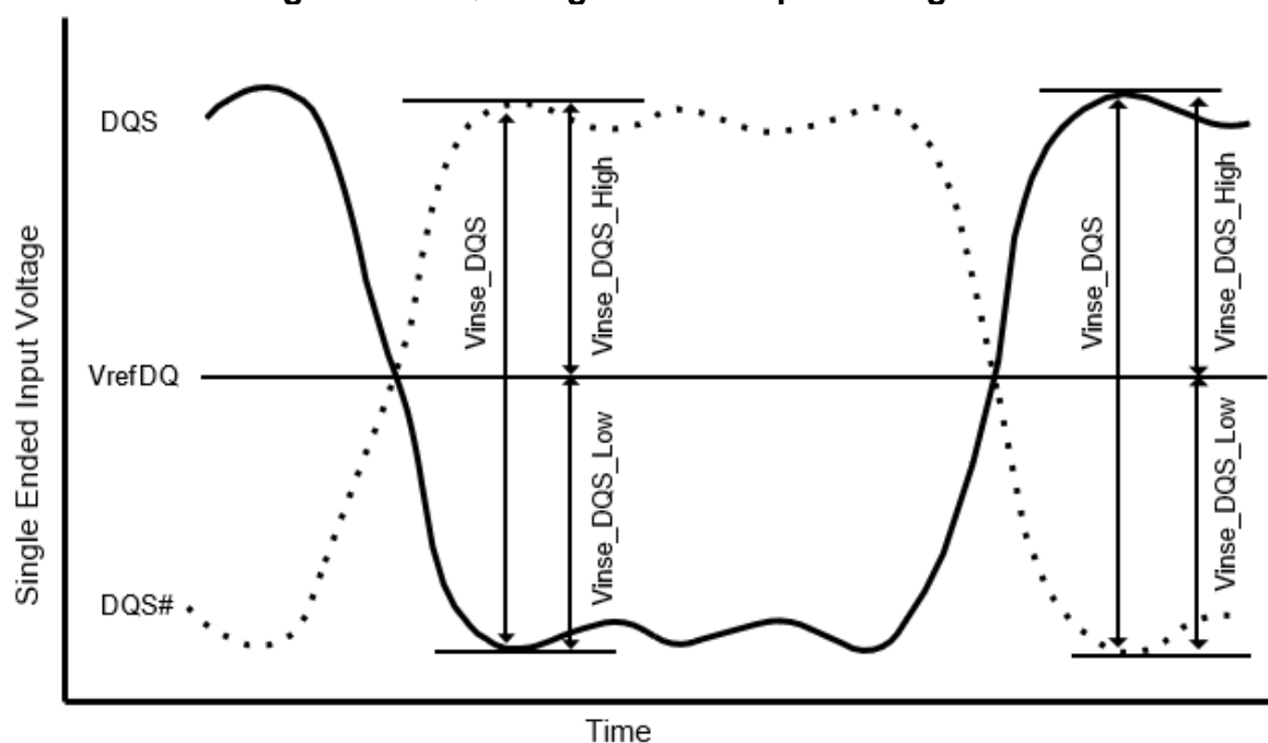
Figure 58. DQS Single-Ended Input Voltage
