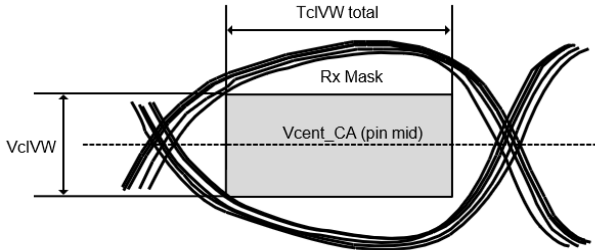
Figure 66. CA Receiver (Rx) mask
