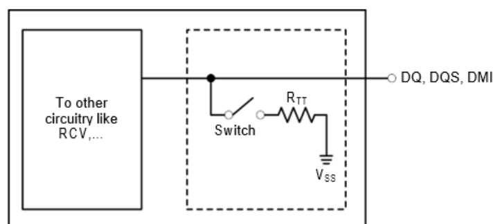
Figure 24. Functional Representation of CA ODT
