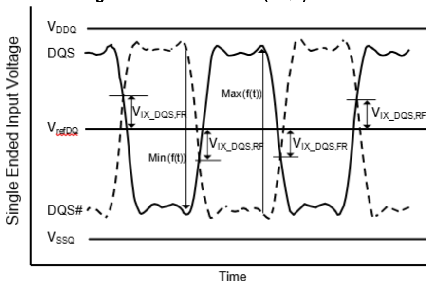
Figure 60. Vix Definition (DQS)
