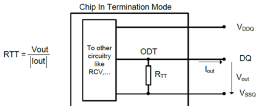
Figure 22. On Die Termination for CA
