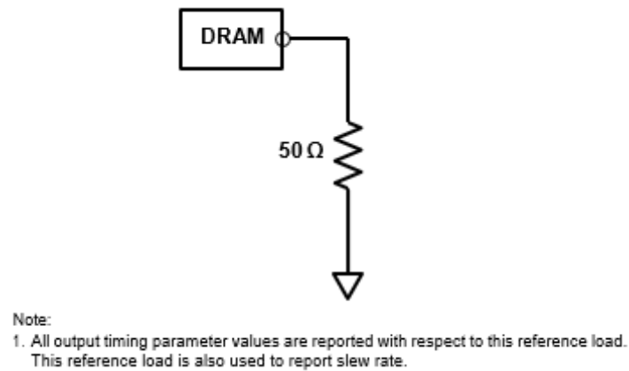
Figure 62. Driver Output Reference Load for Timing and Slew Rate
