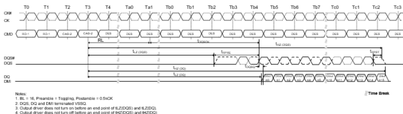
Figure 11. Read Timing
