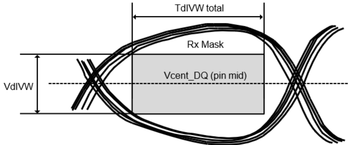
Figure 73. DQ Receiver (Rx) mask
