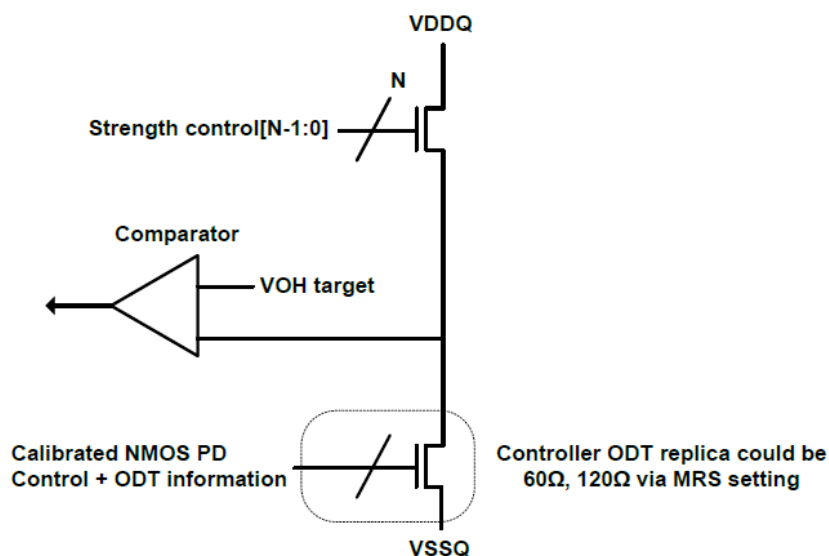
Figure 65. Pull-up calibration
