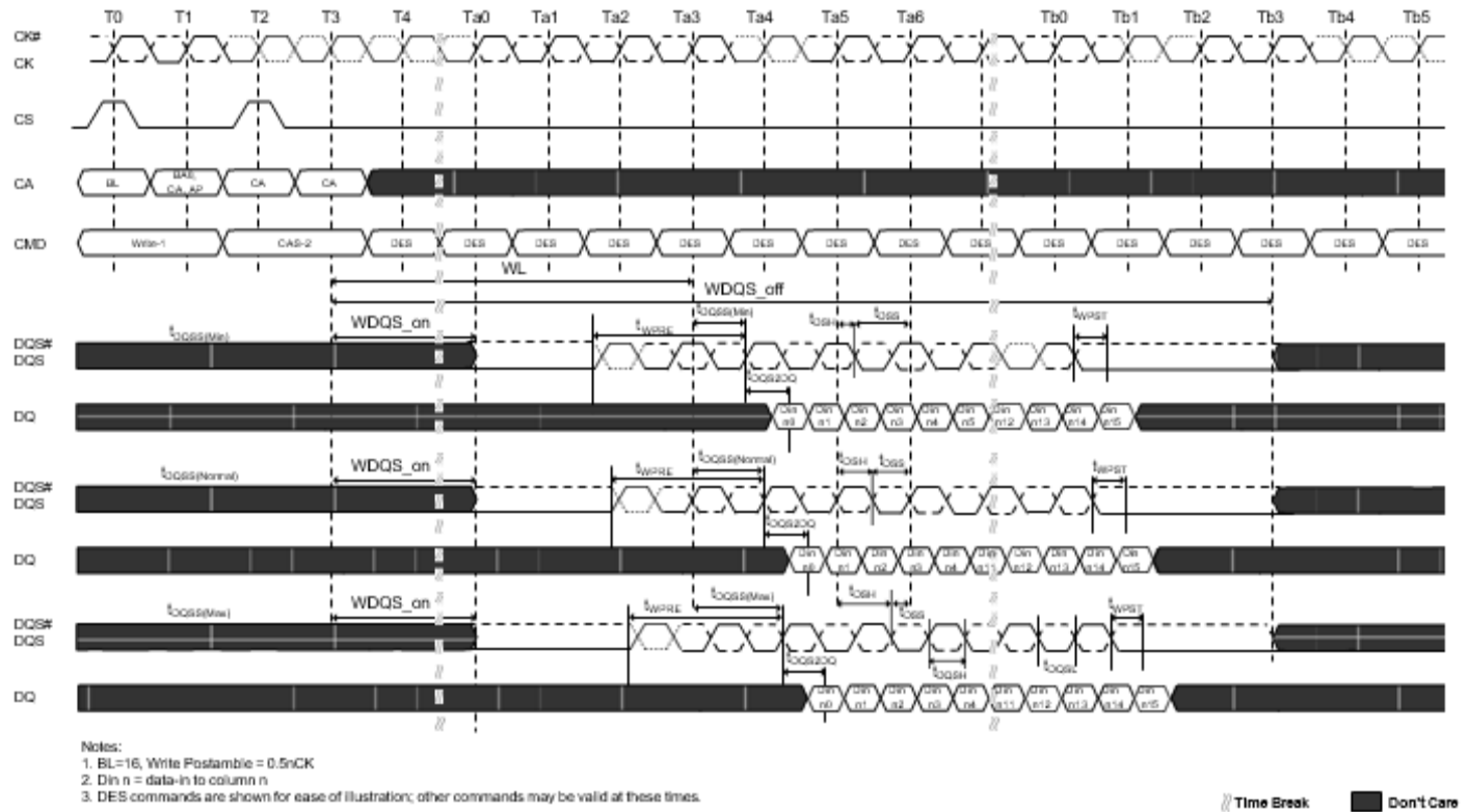
Figure 16. Write Timing
