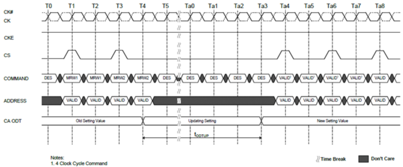
Figure 23. ODT for Command/Address setting update timing in 4 Clock Cycle Command
