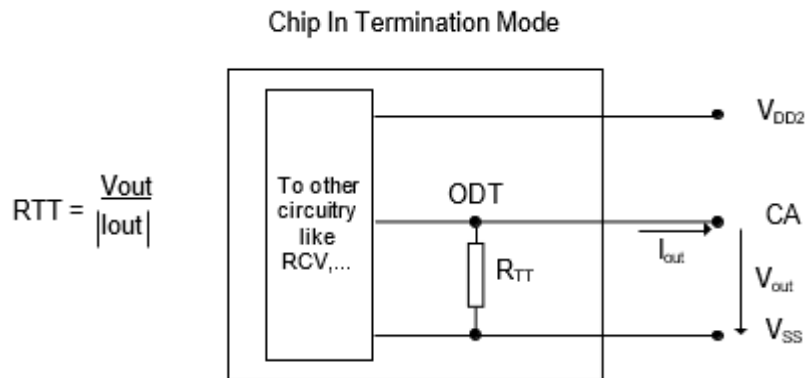
Figure 25. On Die Termination for CA
