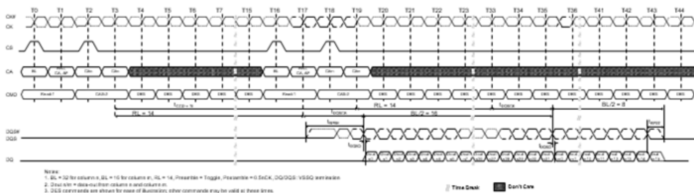
Figure 8. Burst Read Timing
