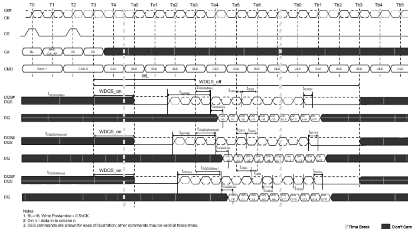
Figure 16. Write Timing
