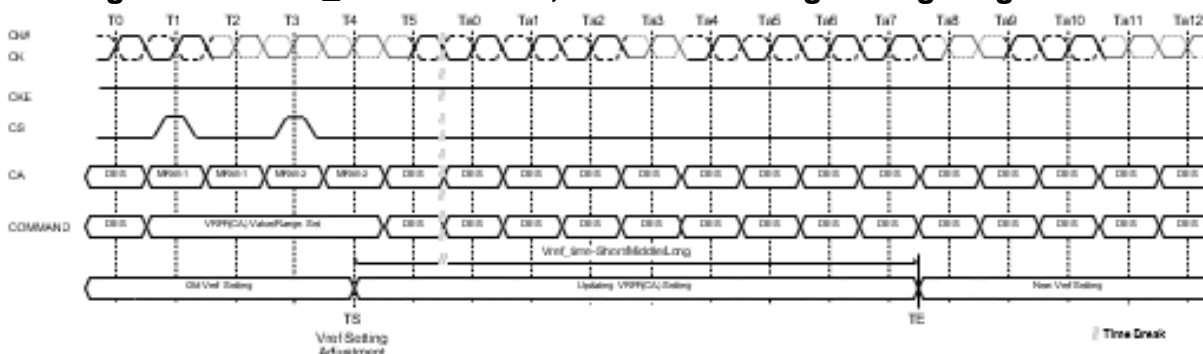
Figure 34. VREF_time for Short, Middle and Long Timing Diagram
