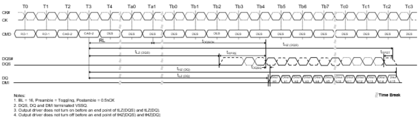
Figure 11. Read Timing
