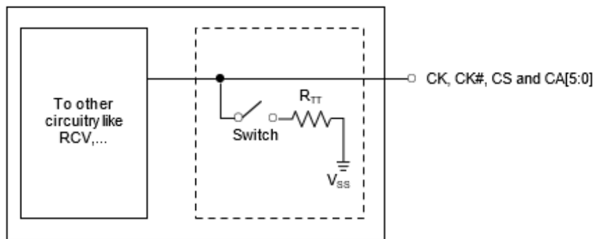
Figure 24. Functional Representation of CA ODT
