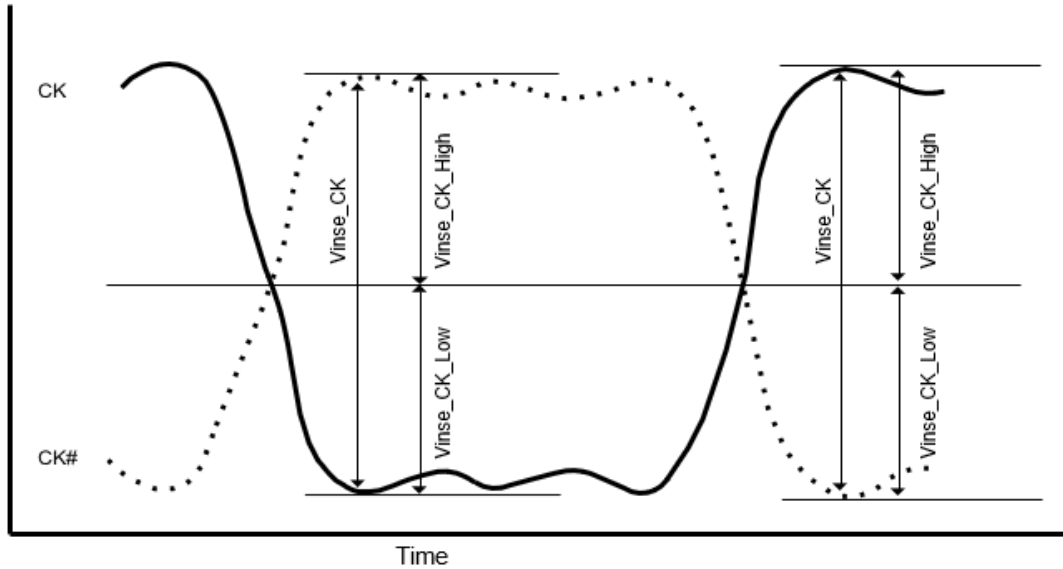
Figure 52. Clock Single-Ended Input Voltage
