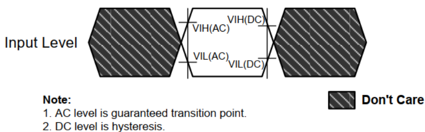
Figure 48. Input AC timing definition for CKE
