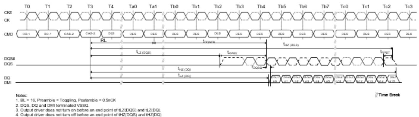
Figure 11. Read Timing
