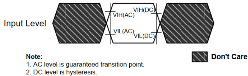
Figure 48. Input AC timing definition for CKE
