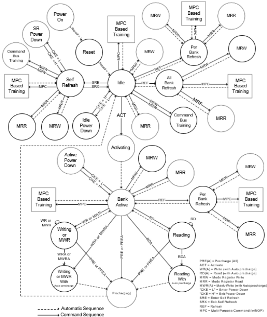
Figure 2. LPDDR4: Simplified Bus Interface State Diagram - Sheet 1
