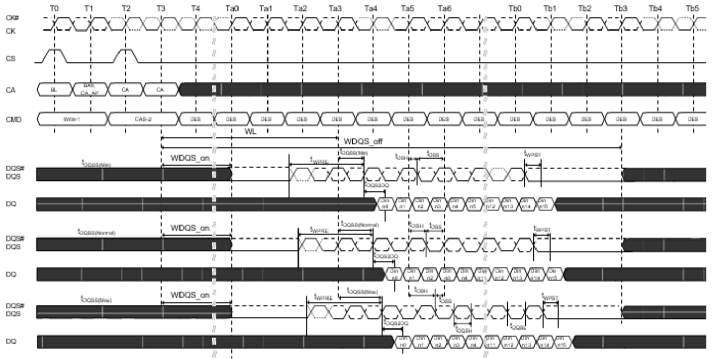
Figure 16. Write Timing
