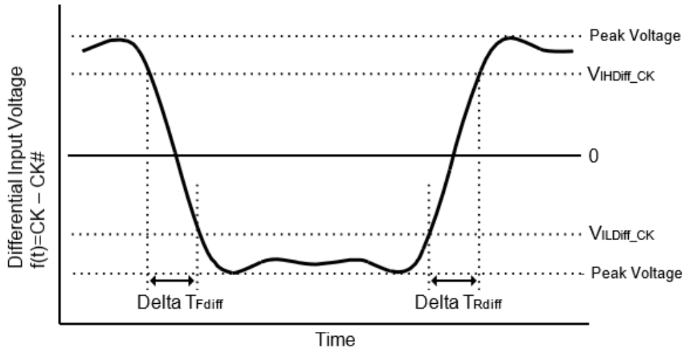
Figure 49. Differential Input Slew Rate Definition for CK, CK#
