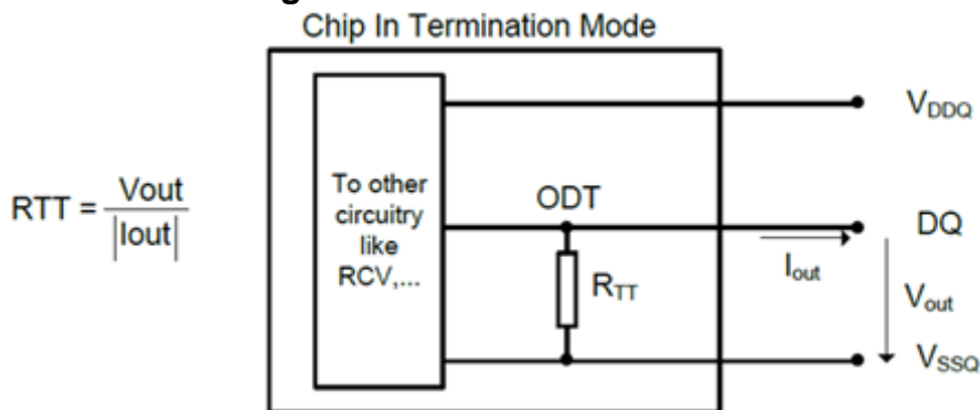
Figure 22. On Die Termination
