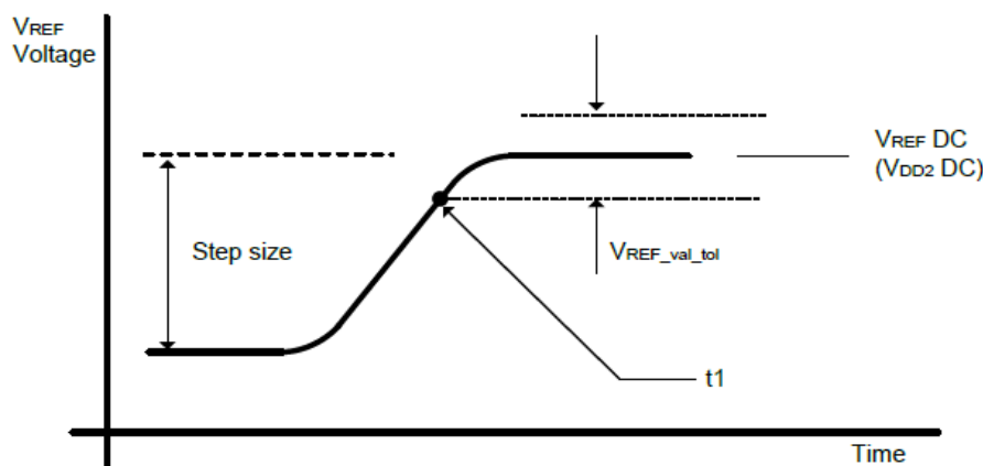
Figure 31. VREF step single step size increment case
