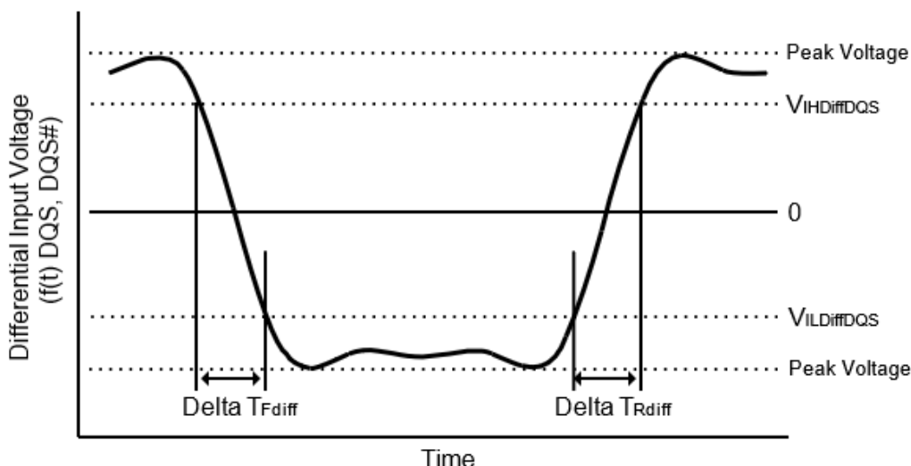
Figure 54. Differential Input Slew Rate Definition for DQS, DQS#
