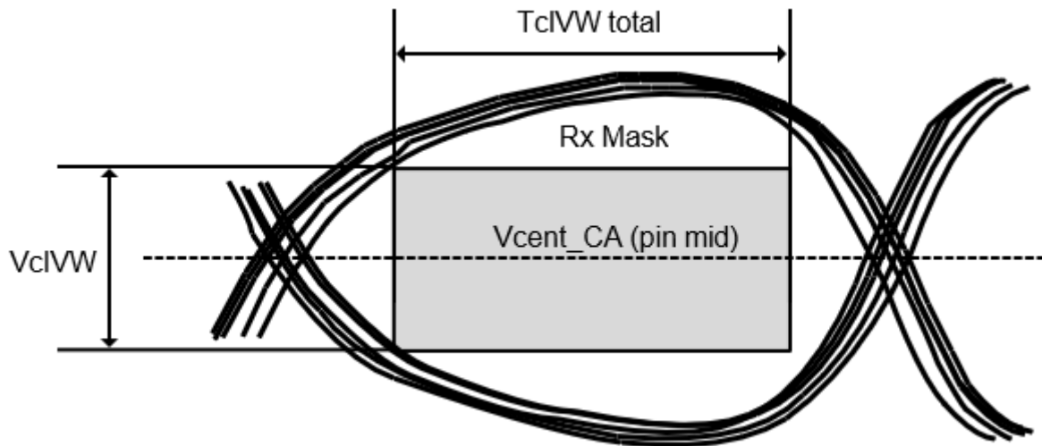
Figure 61. CA Receiver (Rx) mask
