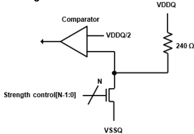
Figure 59. Pull-down calibration
