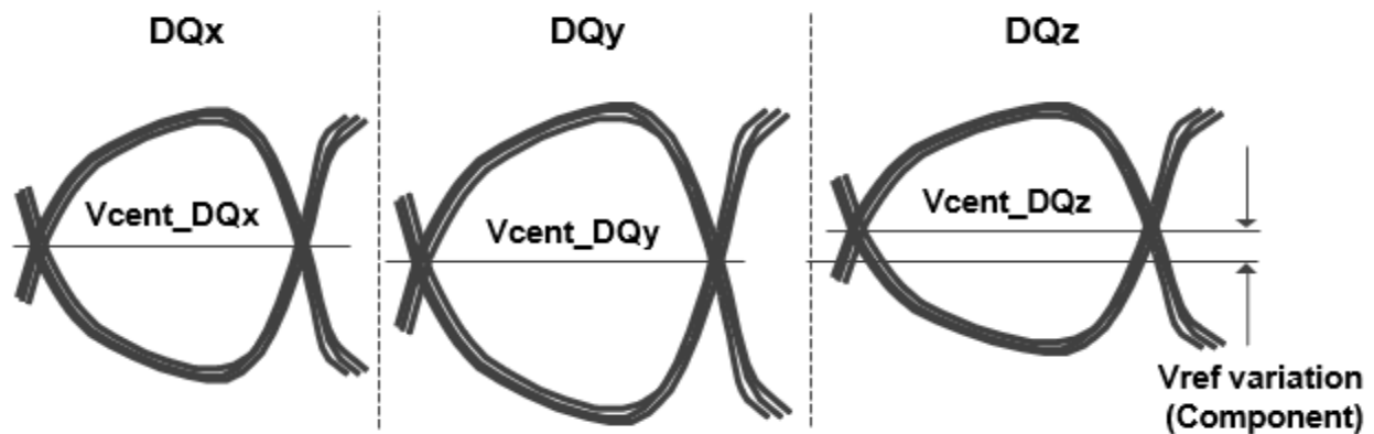
Figure 69. Across Pin Vref DQ Voltage Variation
