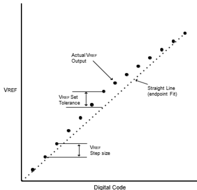
Figure 36. Example of VREF set tolerance (max case only shown) and step size
