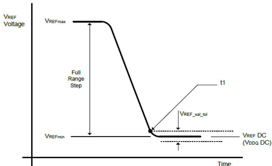
Figure 41. VREF full step from VREFmax to VREFmin case
