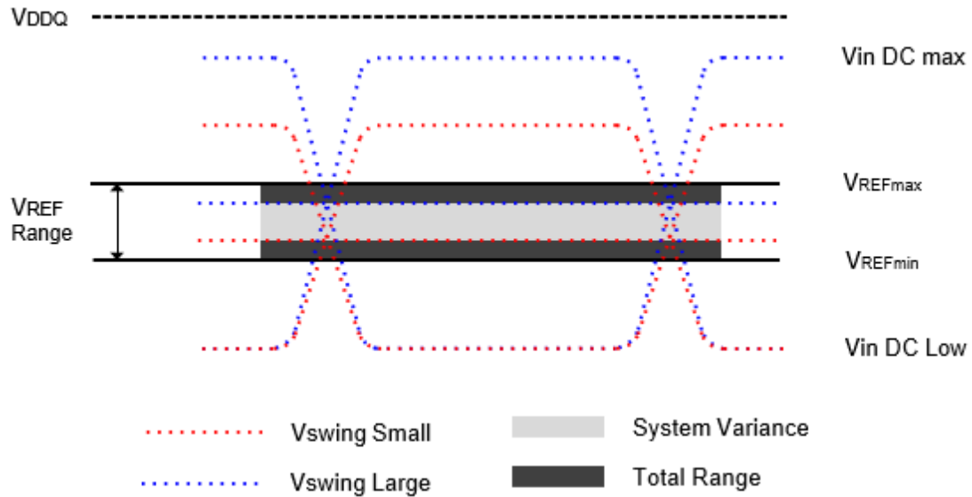
Figure 35. VREF operating range (VREFmin, VREFmax)
