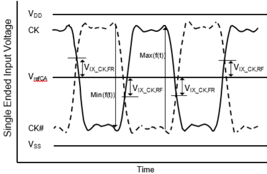
Figure 50. Vix Definition (Clock)
