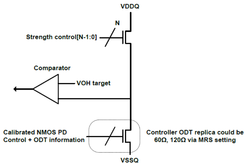
Figure 60. Pull-up calibration
