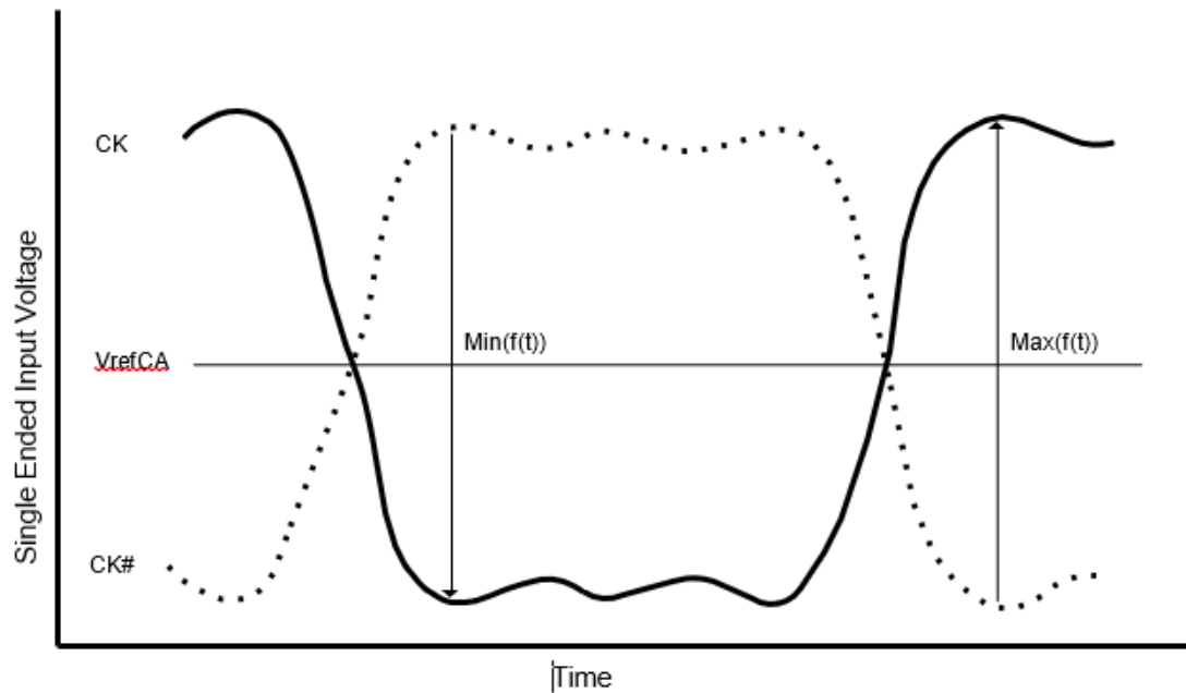
Figure 47. Definition of differential Clock Peak Voltage
