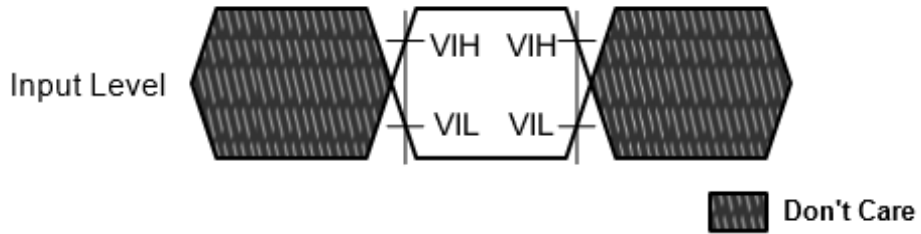
Figure 45. Input AC timing definition for Reset# and ODT_CA
