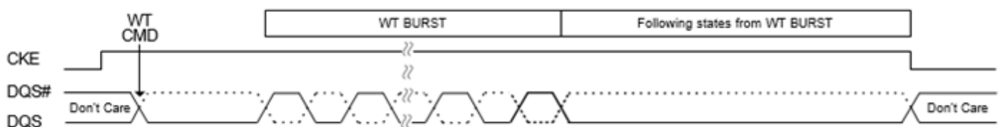
Figure 17. WDQS Control Mode 1 - Read Based Control
