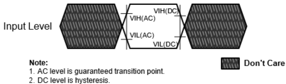
Figure 44. Input AC timing definition for CKE
