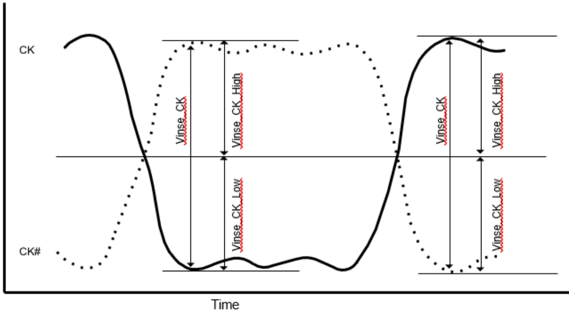
Figure 48. Clock Single-Ended Input Voltage
