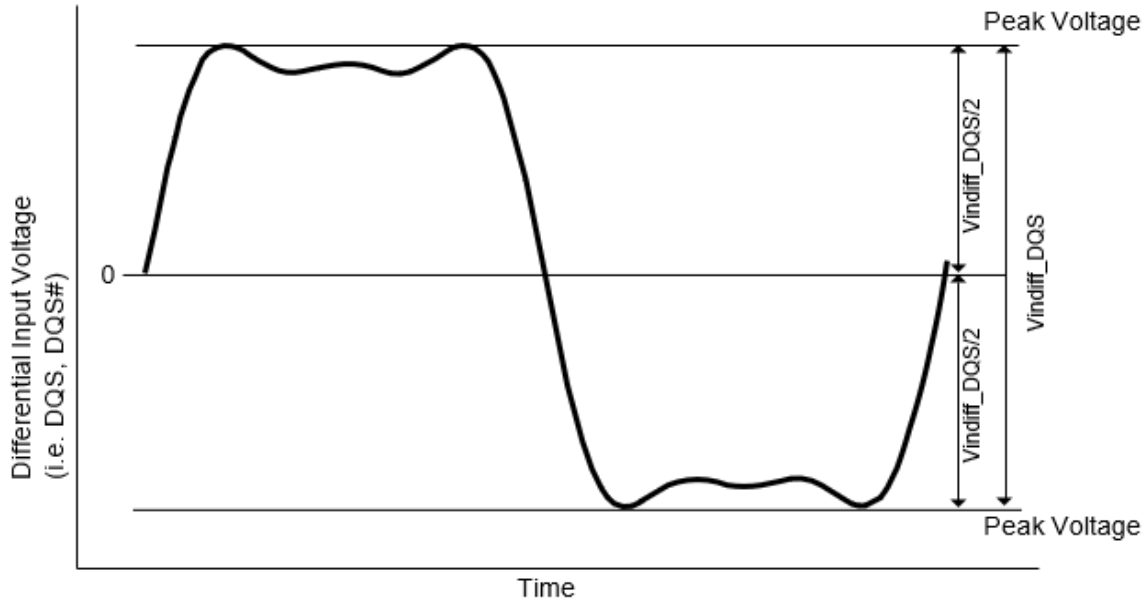
Figure 51. DQS Differential Input Voltage
