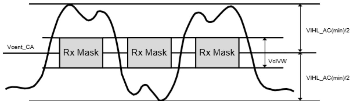
Figure 65. CA VIH L _AC definition (for each input pulse)
