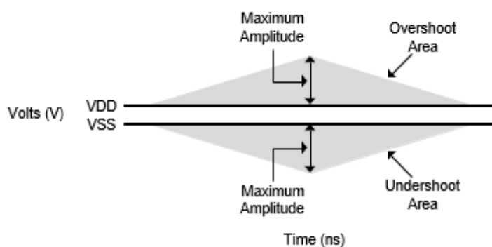
Figure 56. Overshoot and Undershoot Definition
