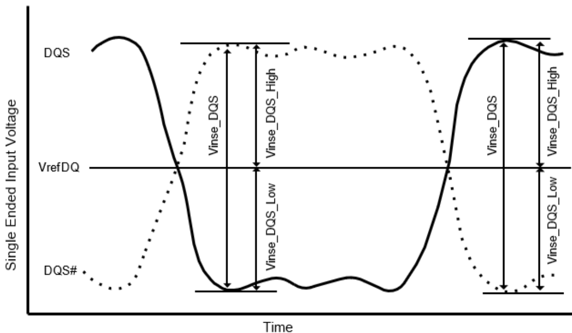
Figure 53. DQS Single-Ended Input Voltage
