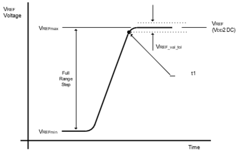
Figure 33. VREF full step from VREFmin to VREFmax case
