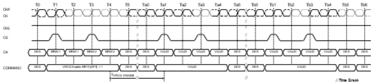
Figure 26. VRCG Enable timing
