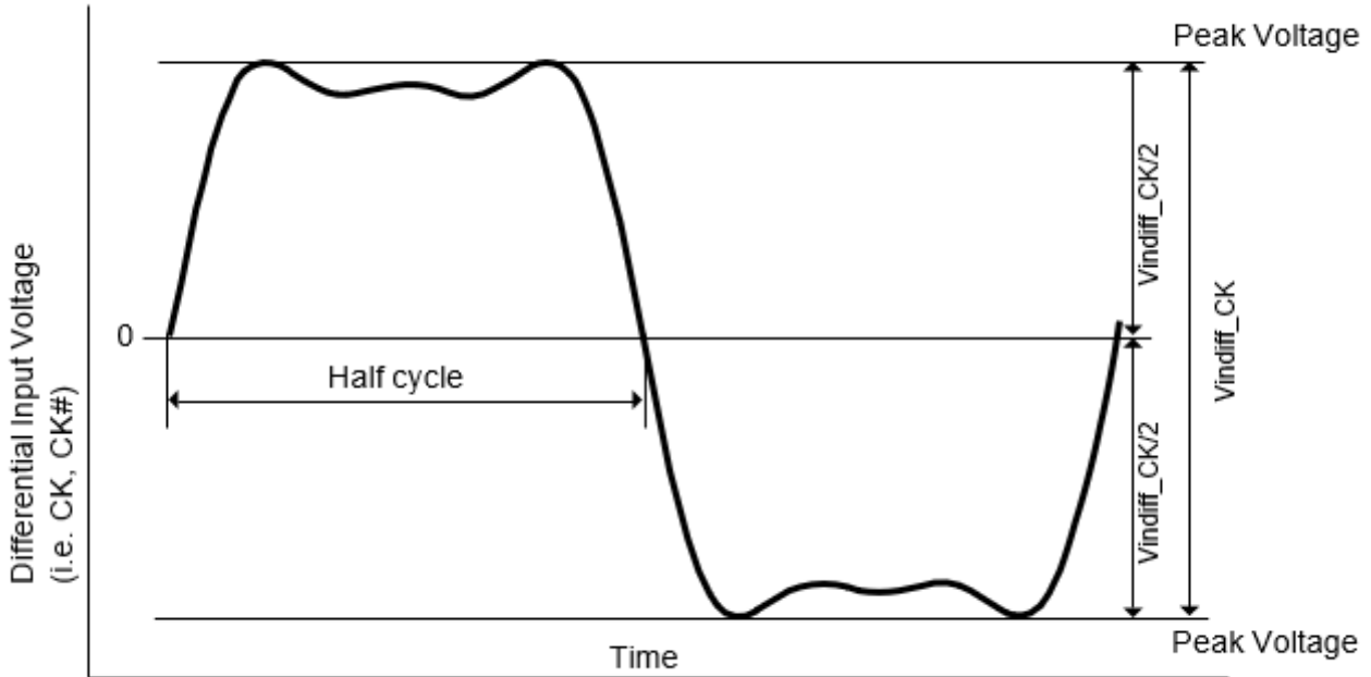
Figure 46. CK Differential Input Voltage
