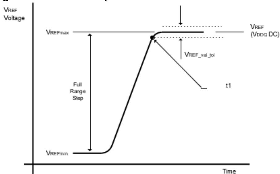
Figure 40. VREF full step from VREFmin to VREFmax case
