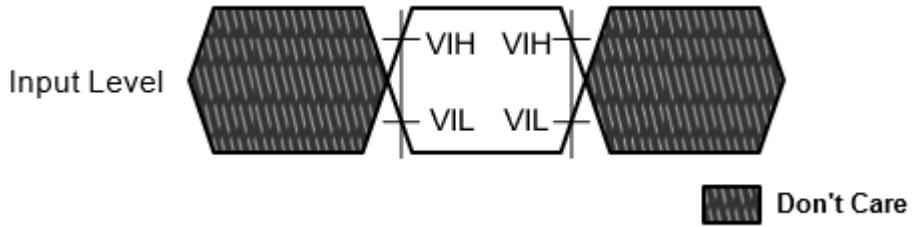
Figure 45. Input AC timing definition for Reset# and ODT_CA
