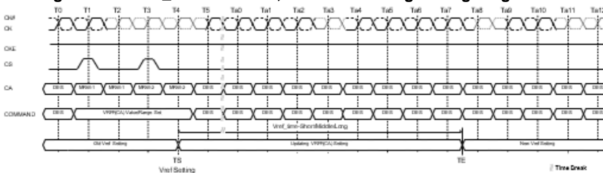
Figure 30. VREF_time for Short, Middle and Long Timing Diagram
