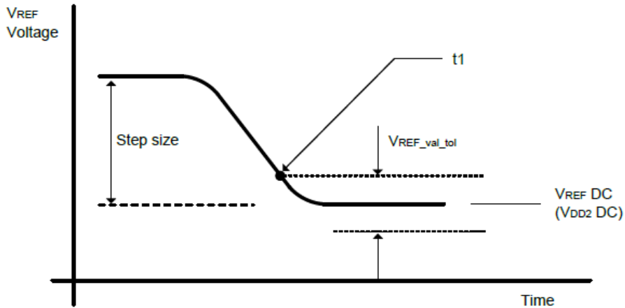
Figure 32. VREF step single step size decrement case
