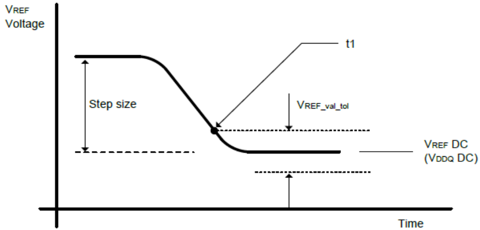
Figure 39. VREF step single step size decrement case
