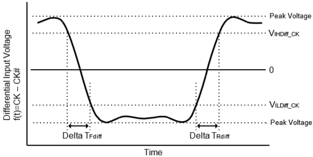
Figure 49. Differential Input Slew Rate Definition for CK, CK#
