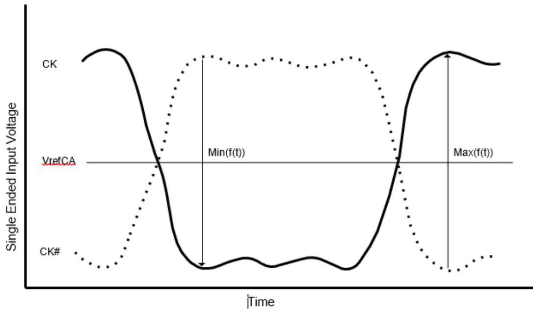
Figure 47. Definition of differential Clock Peak Voltage
