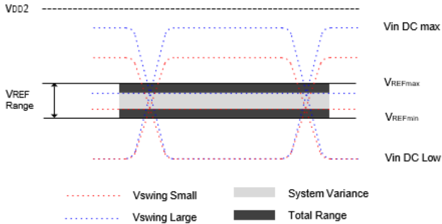
Figure 28. VREF operating range (VREFmin, VREFmax)
