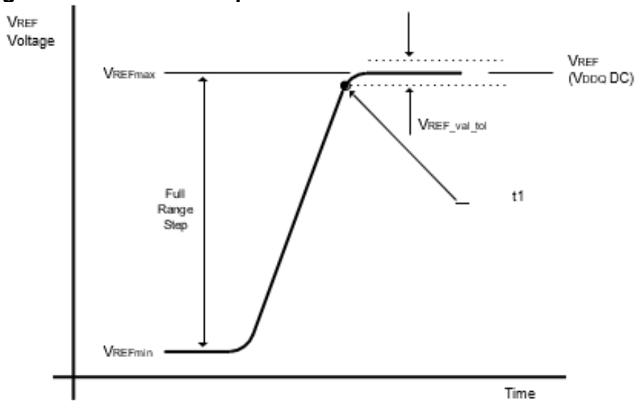
Figure 40. VREF full step from VREFmin to VREFmax case
