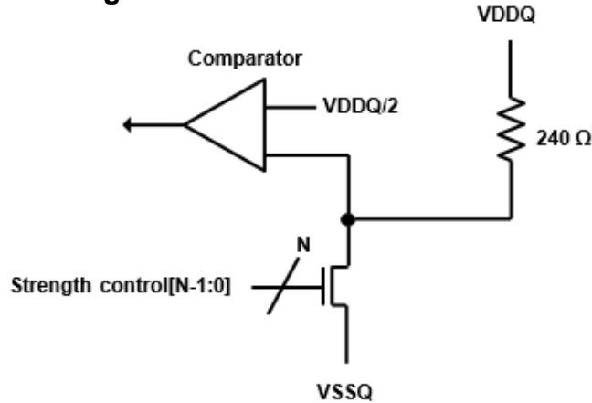
Figure 59. Pull-down calibration
