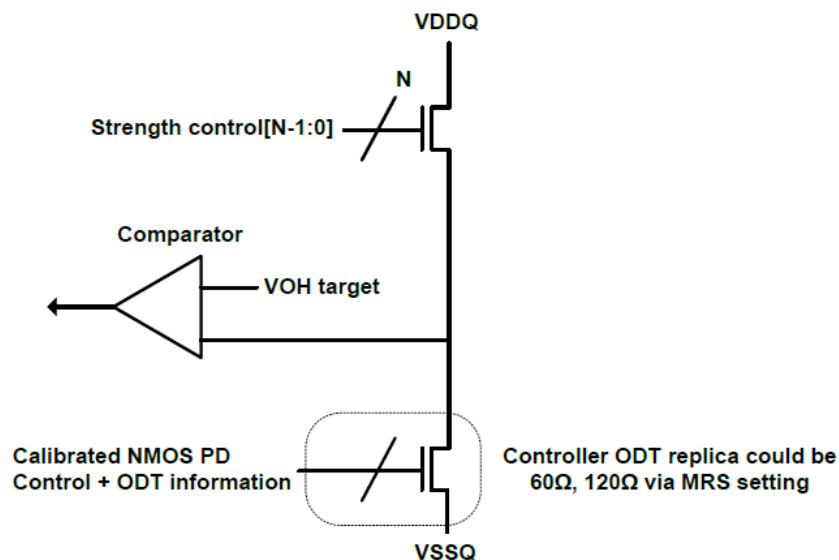
Figure 60. Pull-up calibration
