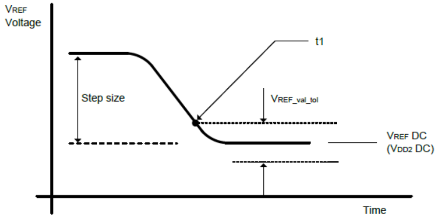
Figure 32. VREF step single step size decrement case
