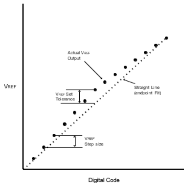
Figure 29. Example of VREF set tolerance (max case only shown) and step size
