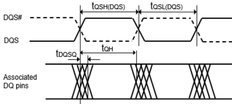
Figure 66. Read data timing definitions t_{QH} and t_{DQSQ} across all DQ signals per DQS group
