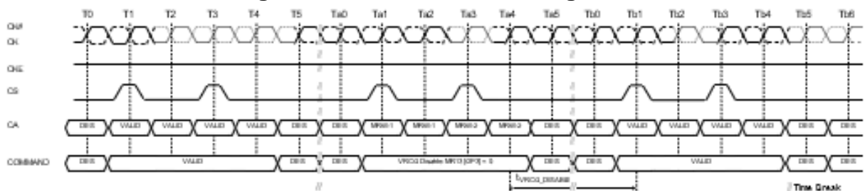
Figure 27. VRCG Disable timing
