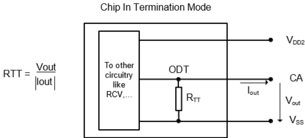
Figure 21. On Die Termination for CA
