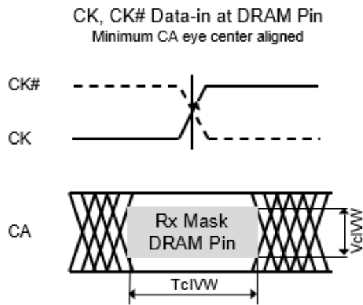
Figure 63. CA Timings at the DRAM Pins
