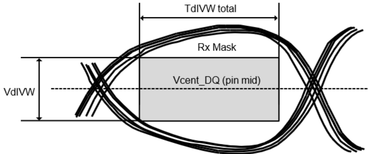
Figure 68. DQ Receiver (Rx) mask
