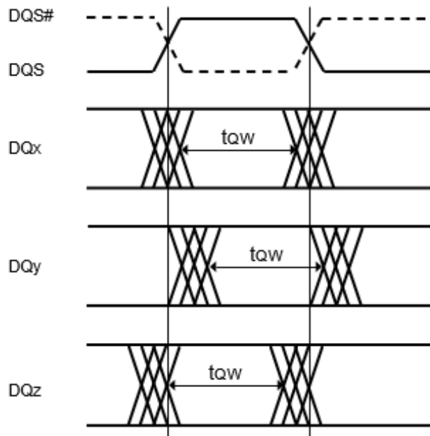
Figure 67. Read Data Timing t_{QW} Valid Window Defined per DQ Signal
