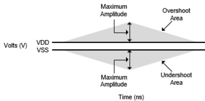
Figure 56. Overshoot and Undershoot Definition
