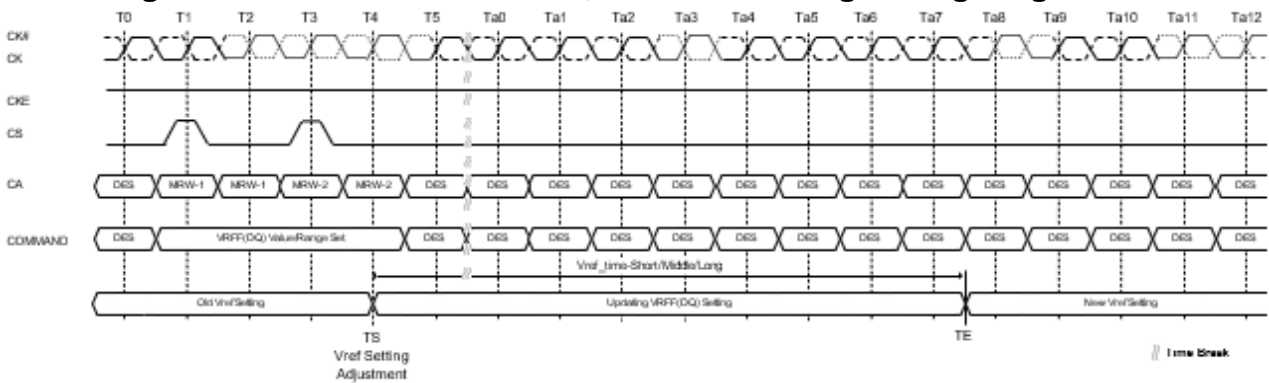
Figure 37. VREF_time for Short, Middle and Long Timing Diagram
