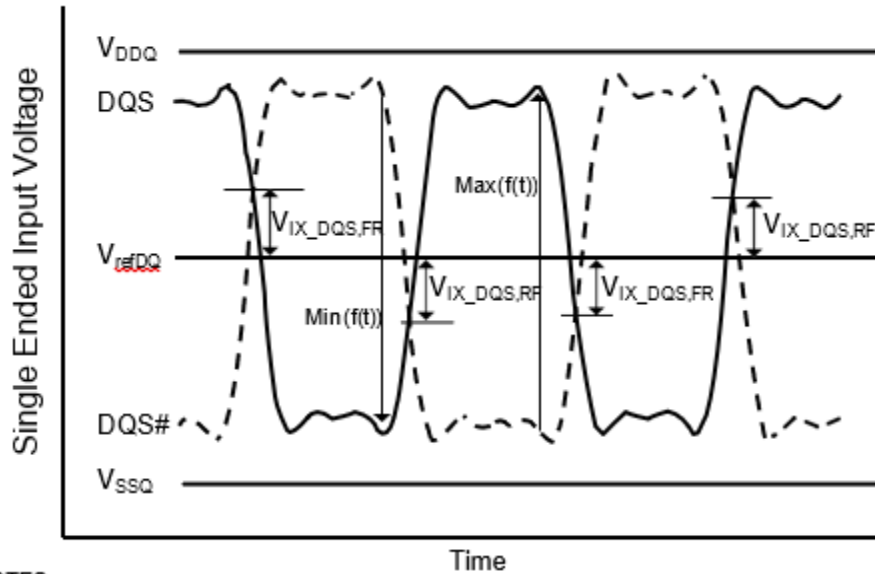
Figure 55. Vix Definition (DQS)
