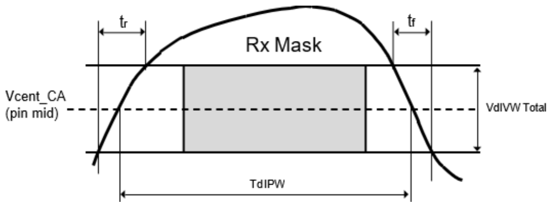
Figure 71. DQ TdIPW and SRIN_dIVW definition (for each input pulse)
