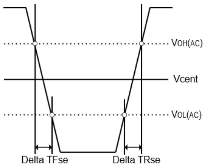
Figure 42. Single Ended Output Slew Rate Definition
