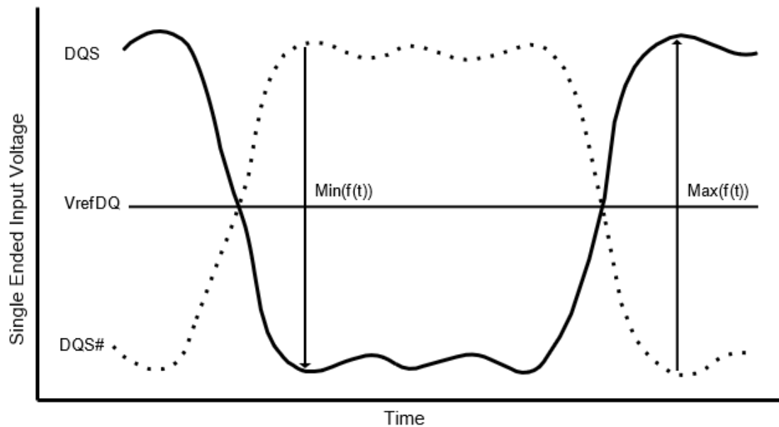
Figure 52. Definition of differential DQS Peak Voltage
