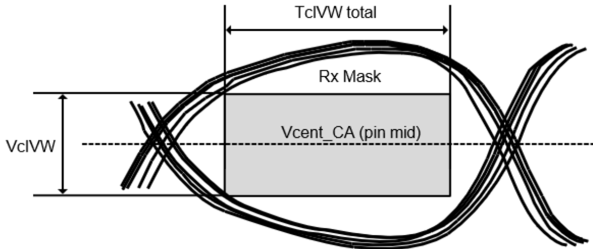
Figure 61. CA Receiver (Rx) mask
