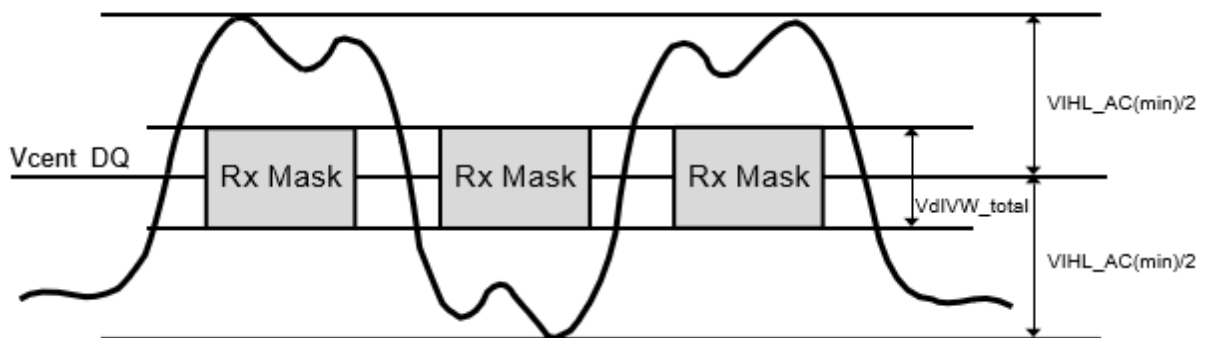
Figure 72. DQ VIH L _AC definition (for each input pulse)
