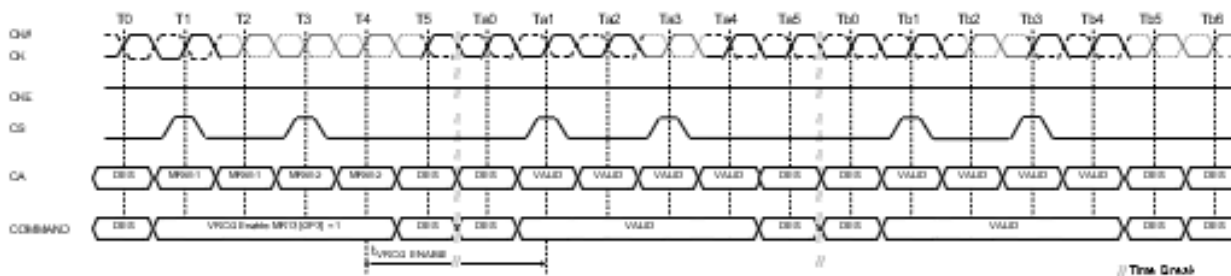
Figure 26. VRCG Enable timing
