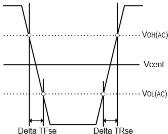
Figure 42. Single Ended Output Slew Rate Definition
