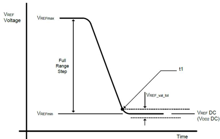
Figure 34. VREF full step from VREFmax to VREFmin case
