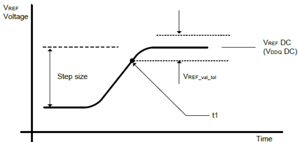
Figure 38. VREF step single step size increment case
