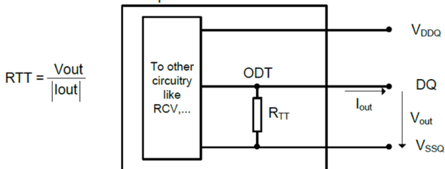
Figure 23. On Die Termination Chip In Termination Mode
