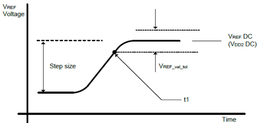
Figure 35. VREF step single step size increment case
