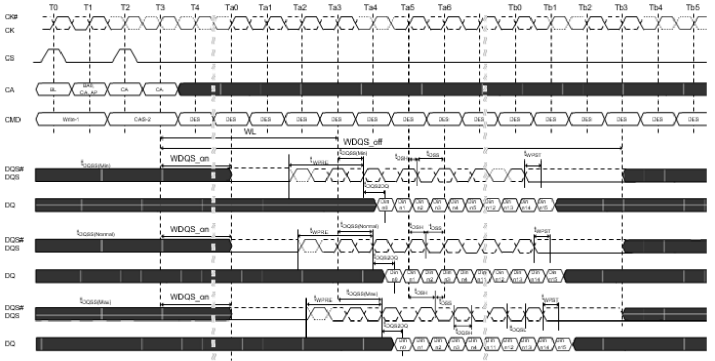
Figure 16. Write Timing
