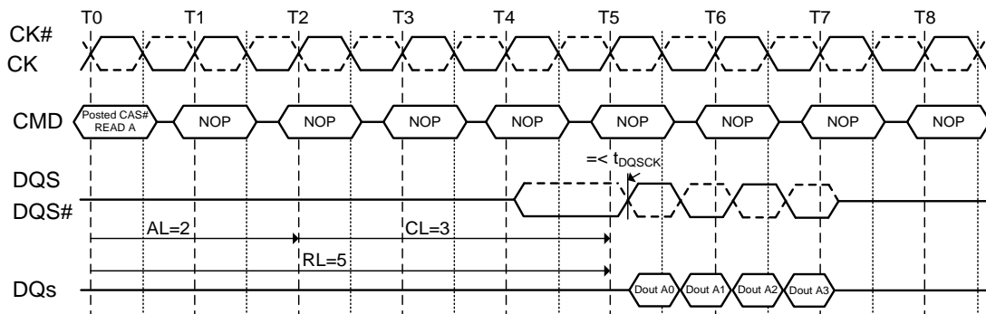
Figure 21. Burst read operation: RL=5 (AL=2, CL=3, BL=4)
