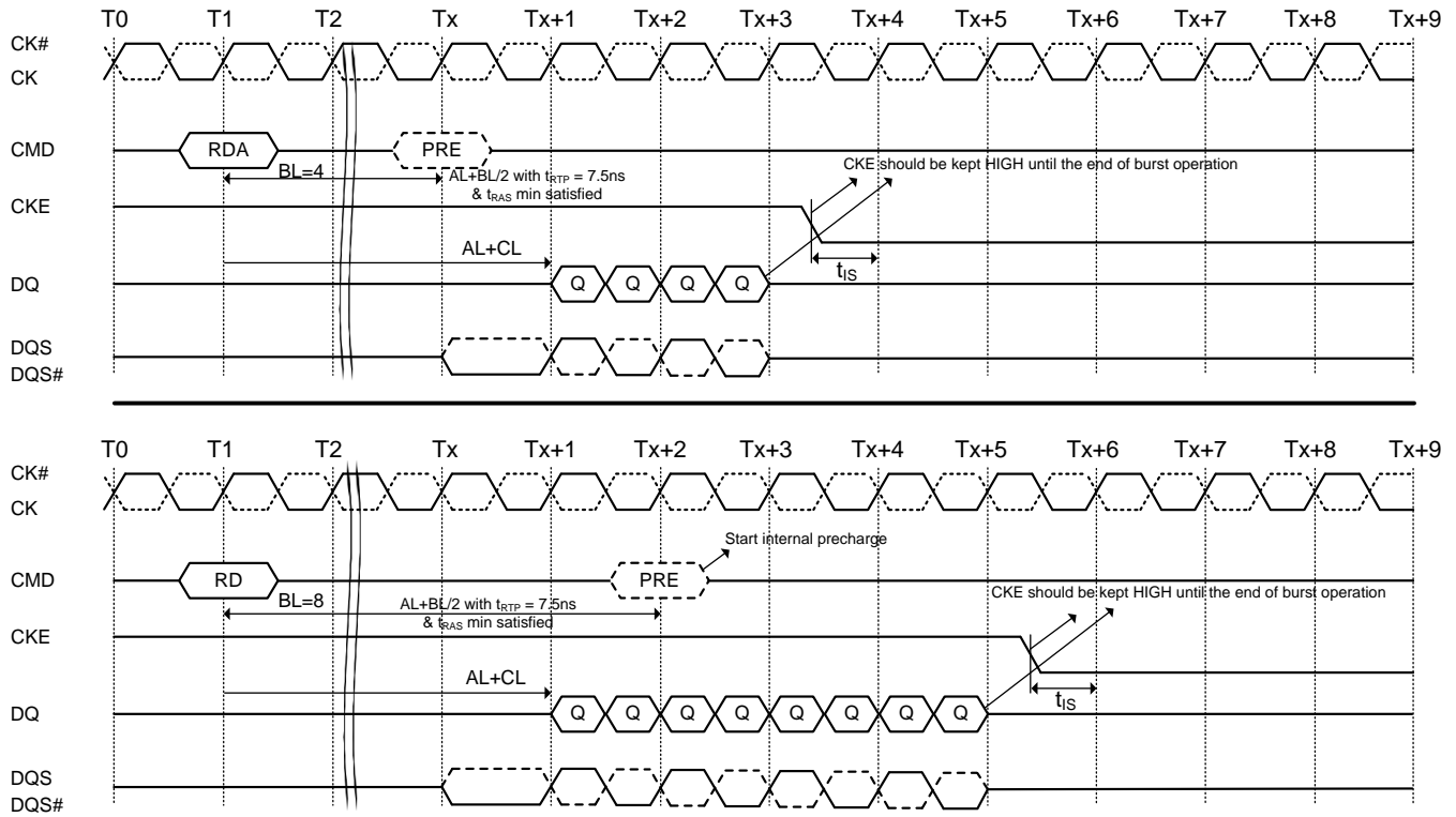
Figure 52. Read with autoprecharge to power-down entry
