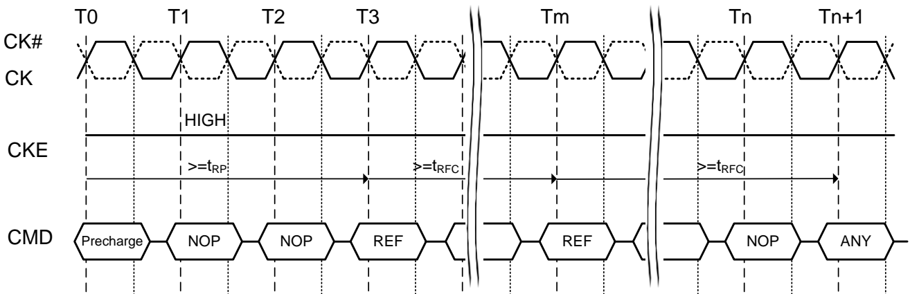
Figure 46. Refresh command
