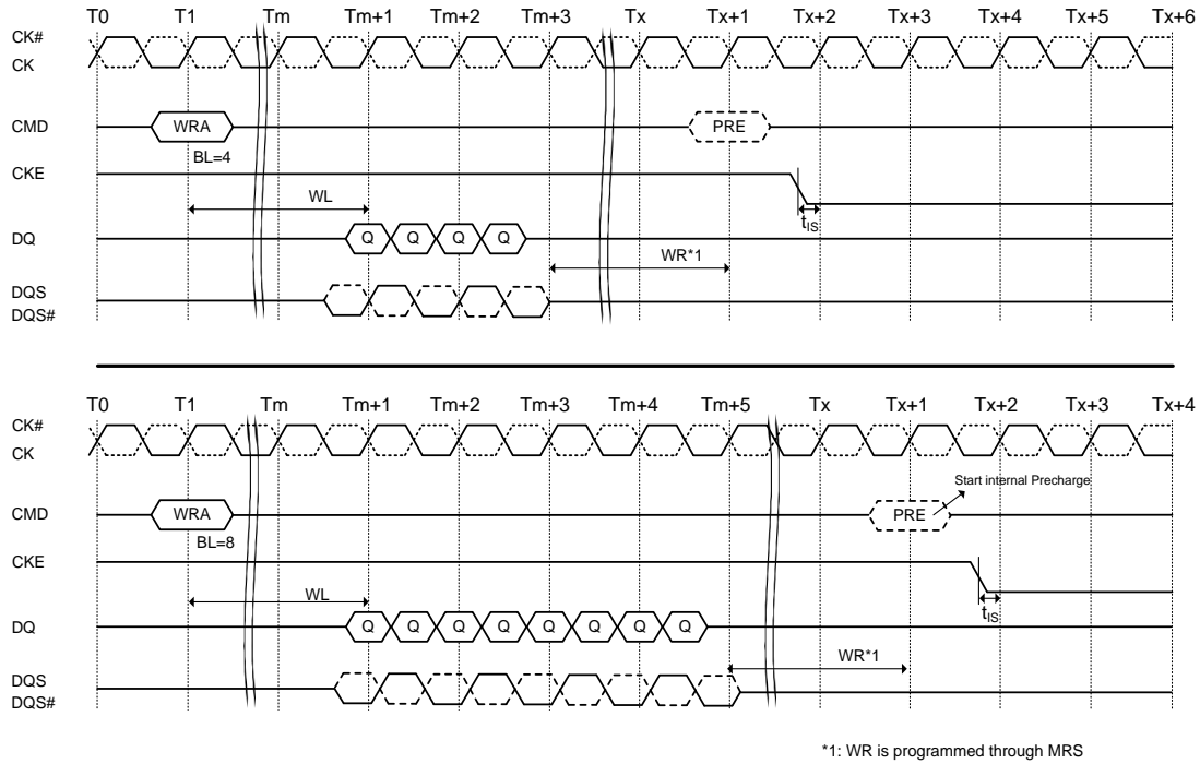
Figure 54. Write with autoprecharge to power-down entry
