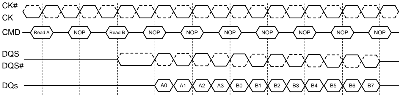
Figure 25. Read burst interrupt timing: (CL=3, AL=0, RL=3, BL=8)
