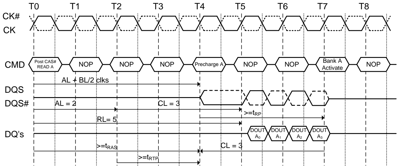
Figure 35. Burst read operation followed by precharge: (RL=5, AL=2, CL=3, BL=4, t_{RTP} \leq 2 clocks)
