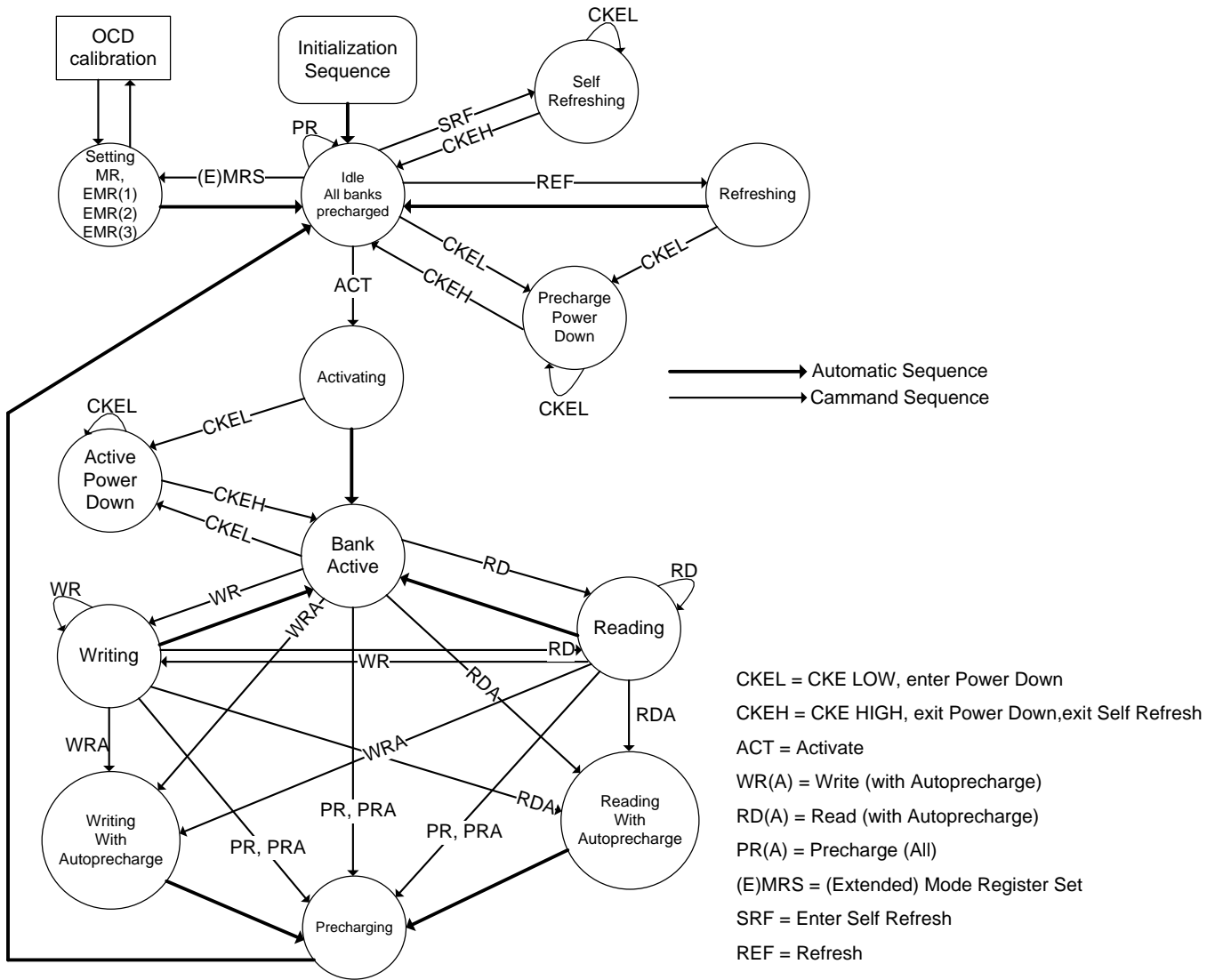
Figure 3. State Diagram
