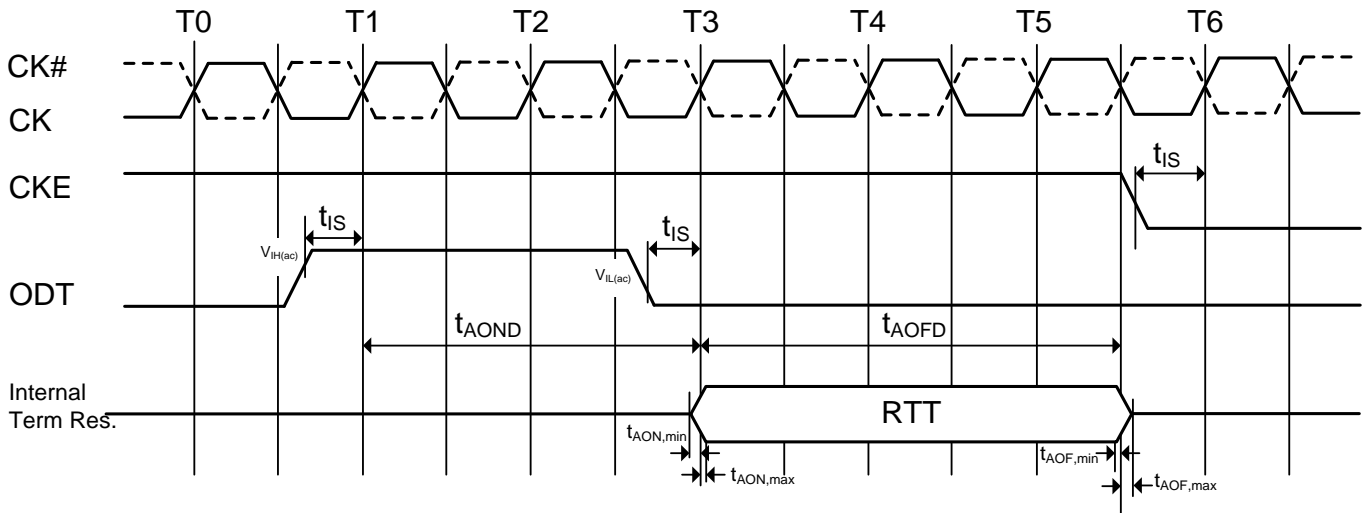
Figure 14. ODT timing for power-down mode
