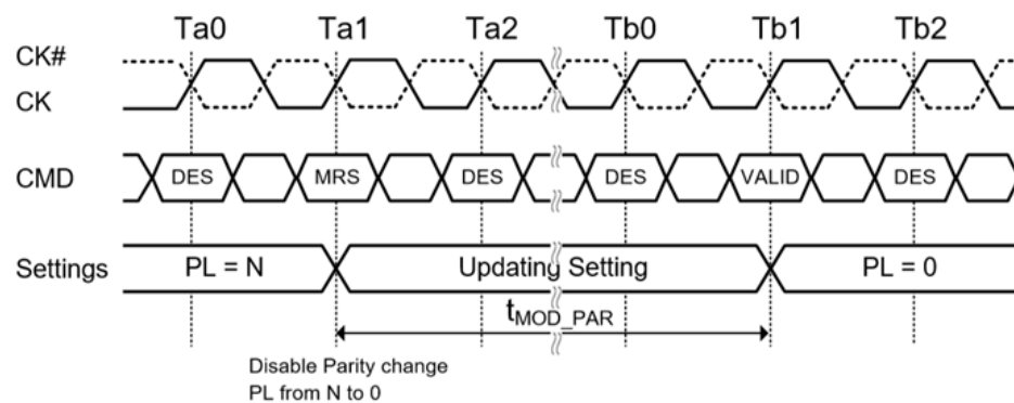
Figure 65. Parity exit timing example - tMOD_PAR
