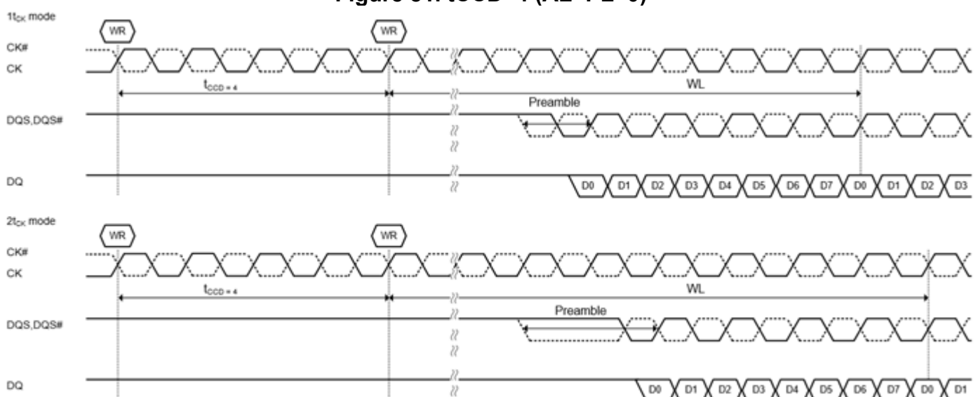
Figure 81. t_{CCD}=4 (AL=PL=0)
