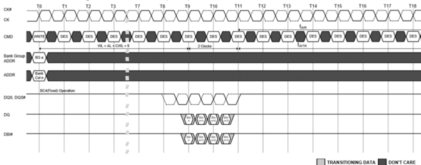
Figure 155. WRITE (BC4) Fixed with 1tCK Preamble and DBI
