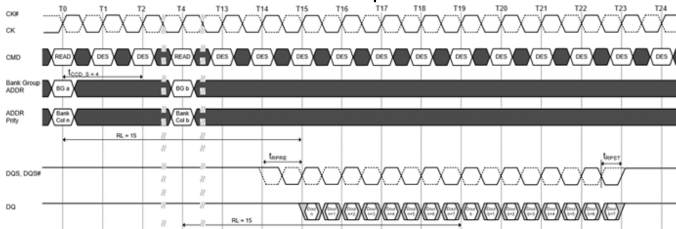
Figure 123. Consecutive READ (BL8) with 1tCK Preamble and CA Parity in Different Bank Group
