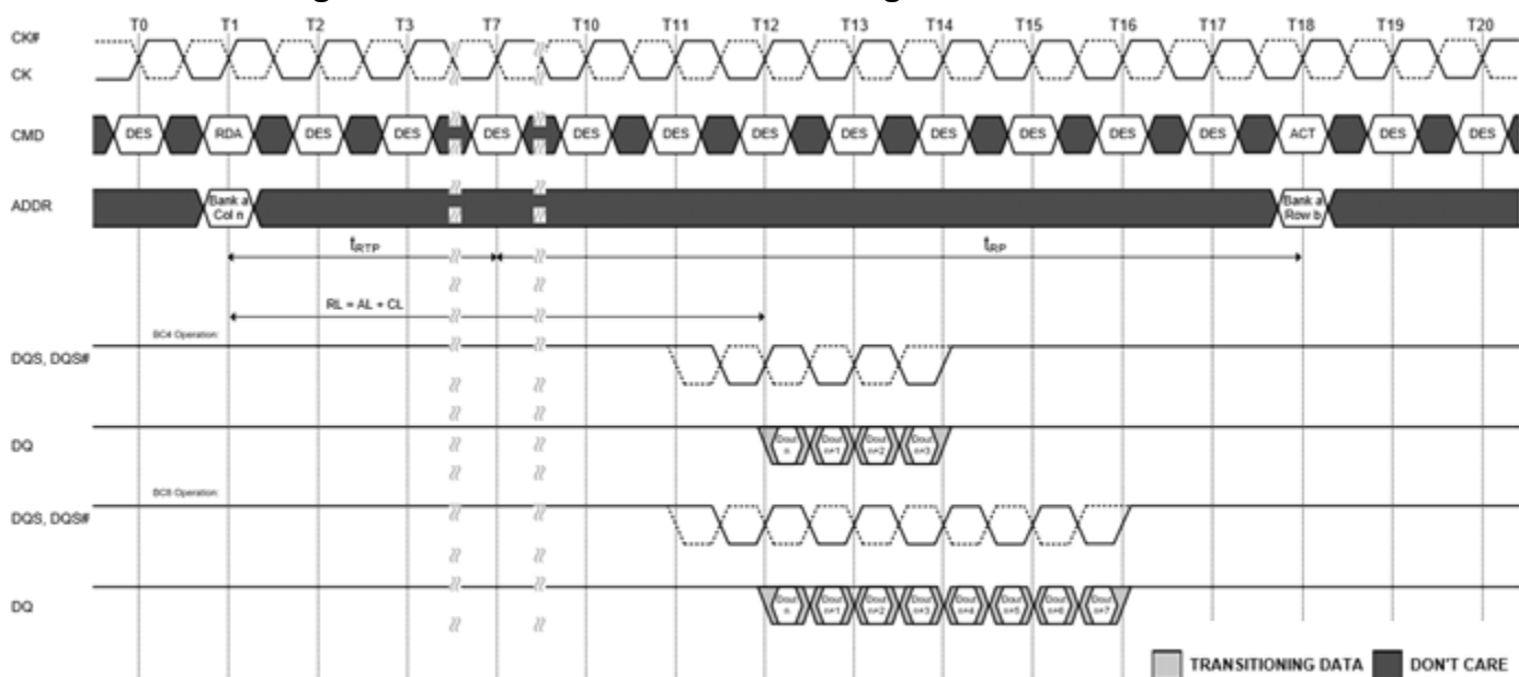
Figure 120. READ with Auto Precharge and 1tCK Preamble
