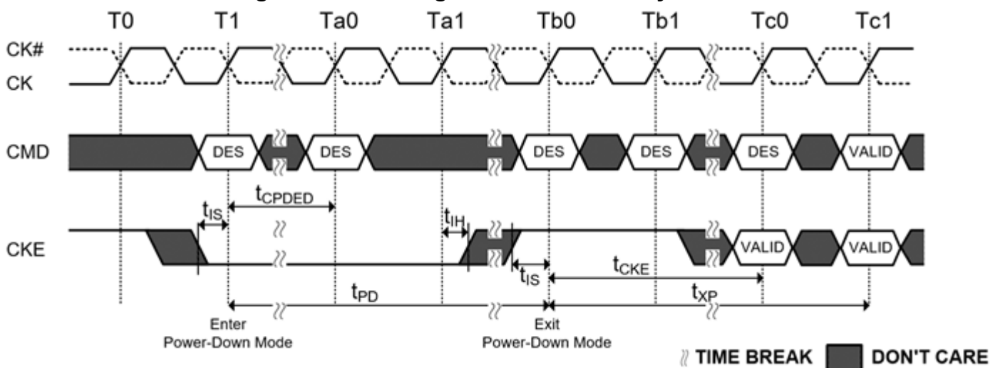
Figure 32. Precharge Power-Down Entry and Exit
