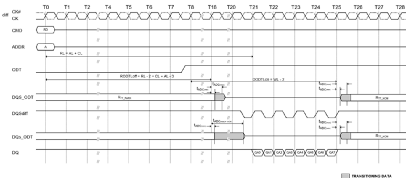
Figure 175. Example: CL=11, PL=0; AL=CL-1=10; RL=AL+PL+CL=21; CWL=9; DODTLon=AL+CWL-2=17; DODTLoff=AL+CWL-2=17; 2tCK preamble)
