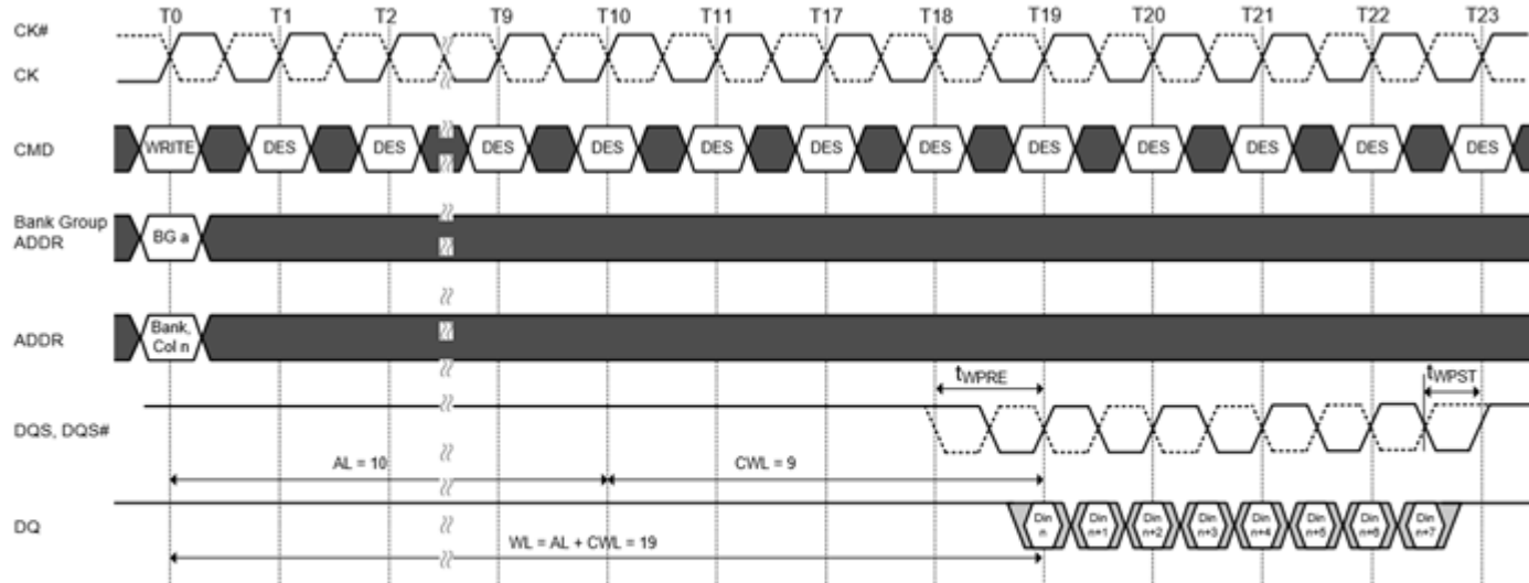
Figure 134. WRITE Burst Operation WL = 19 (AL = 10, CWL = 9, BL8)
