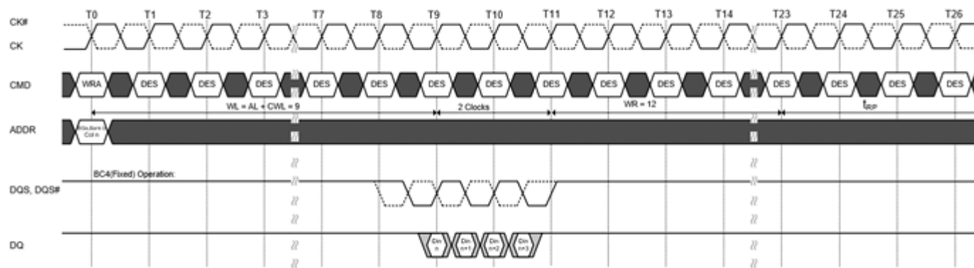
Figure 153. WRITE (BC4) Fixed with Auto PRECHARGE Operation and 1tCK Preamble
