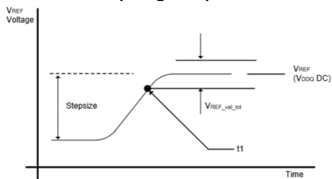
Figure 50. VREF step single stepsize increment case
