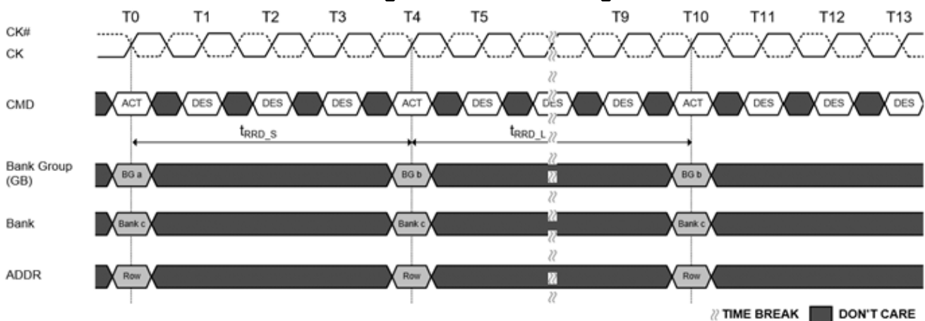
Figure 76. tRRD Timing
