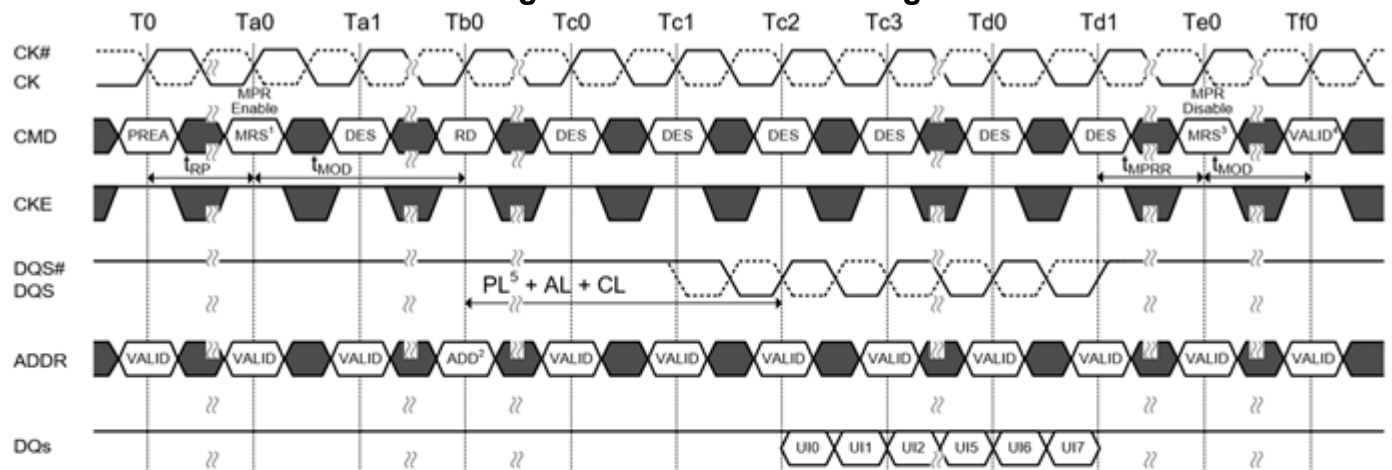
Figure 66. MPR Read Timing
