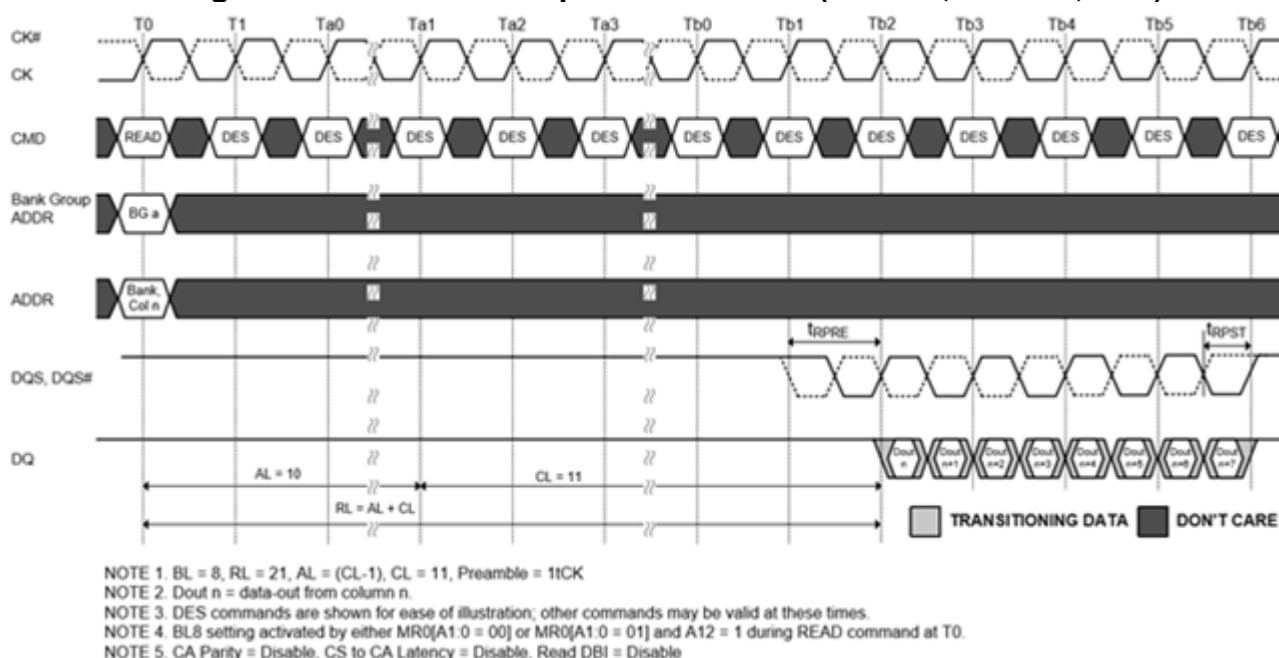
Figure 96. READ Burst Operation RL = 21 (AL = 10, CL = 11, BL8)
