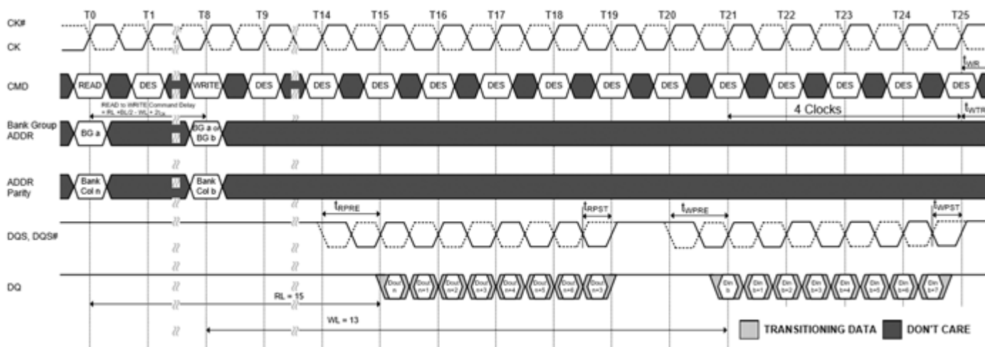
Figure 124. READ (BL8) to WRITE (BL8) with 1tCK Preamble and CA parity in Same or Different Bank Group
