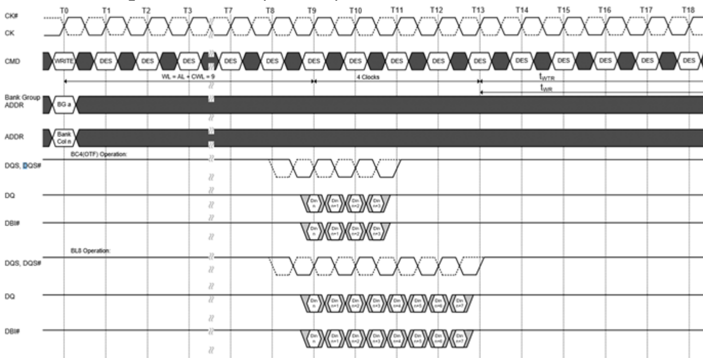
Figure 154. WRITE (BL8/BC4) OTF with 1tCK Preamble and DBI
