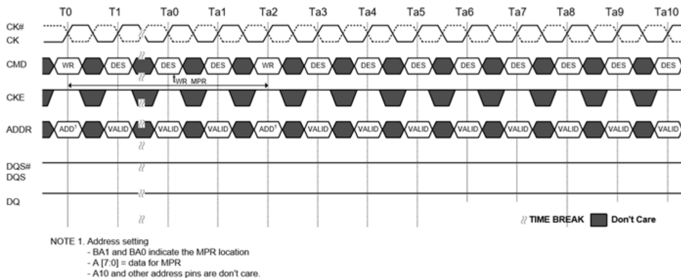
Figure 70. MPR Back to Back Write Timing
