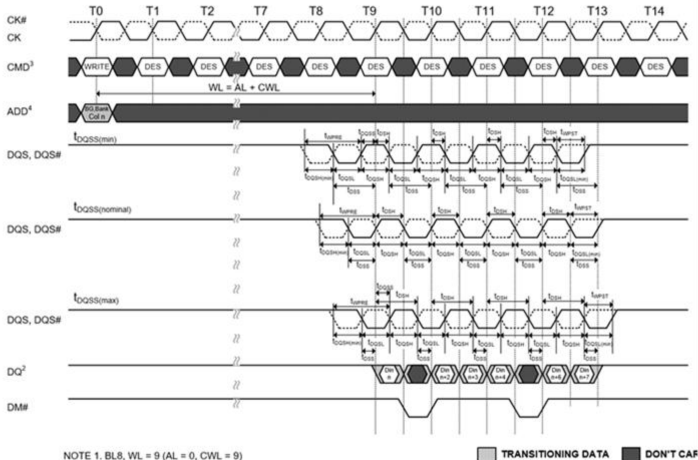
Figure 129. Write Timing Definition and Parameters with 1tCK Preamble
