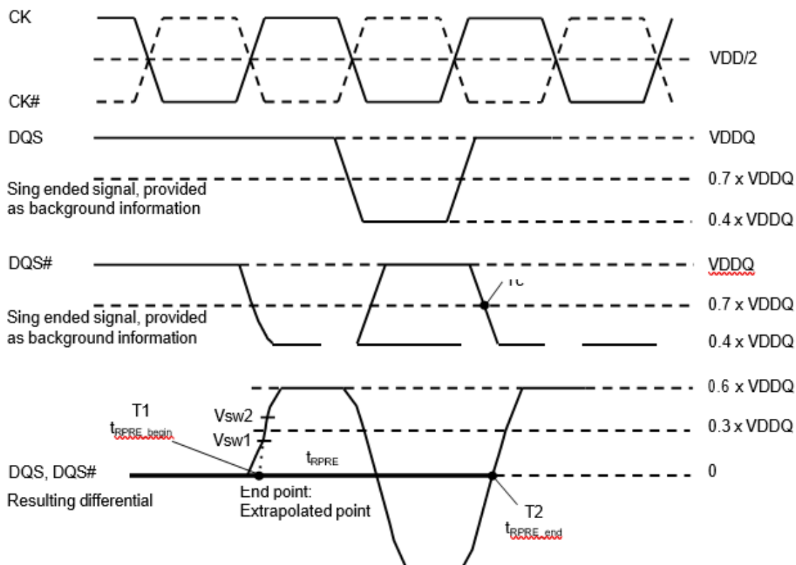
Figure 93. Method for calculating tRPRE transitions and endpoints
