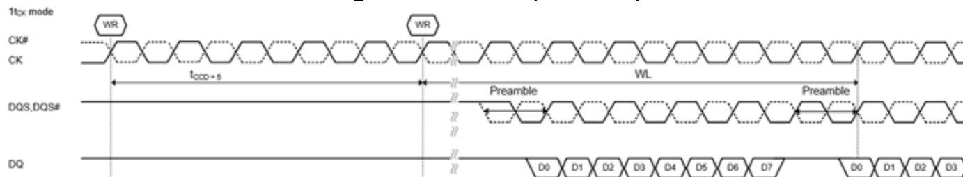
Figure 82. t CCD =5 (AL=PL=0)
