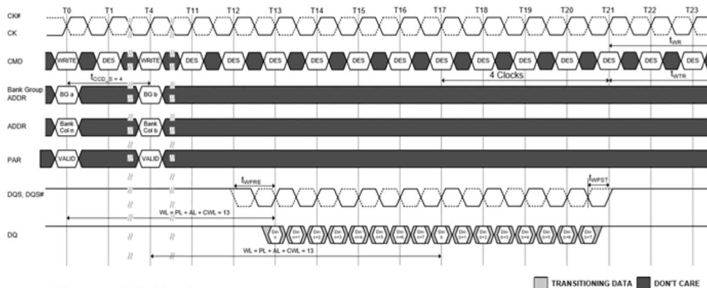
Figure 156. Consecutive WRITE (BL8) with 1tCK Preamble and CA Parity in Different Bank Group
