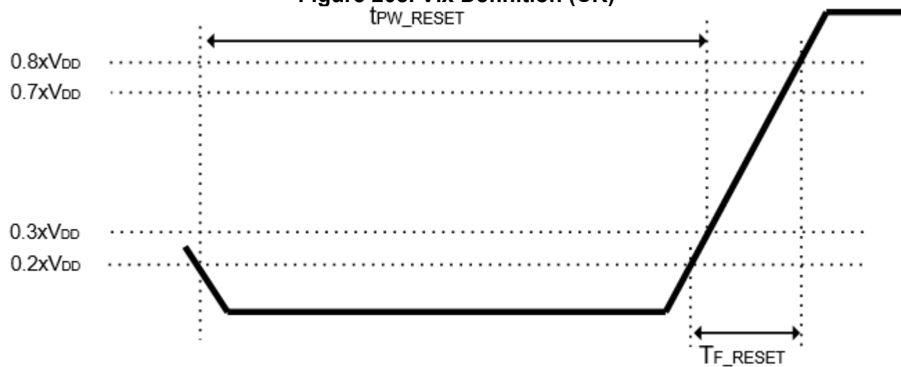
Figure 208. Vix Definition (CK)
