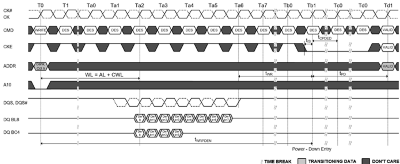
Figure 31. Power-Down Entry After Write
