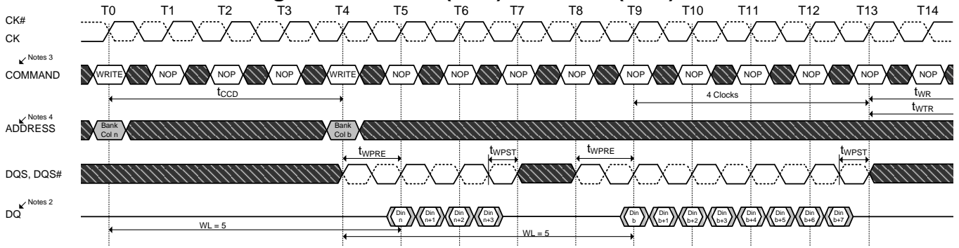
Figure 54. WRITE (BC4) to WRITE (BC8) OTF
