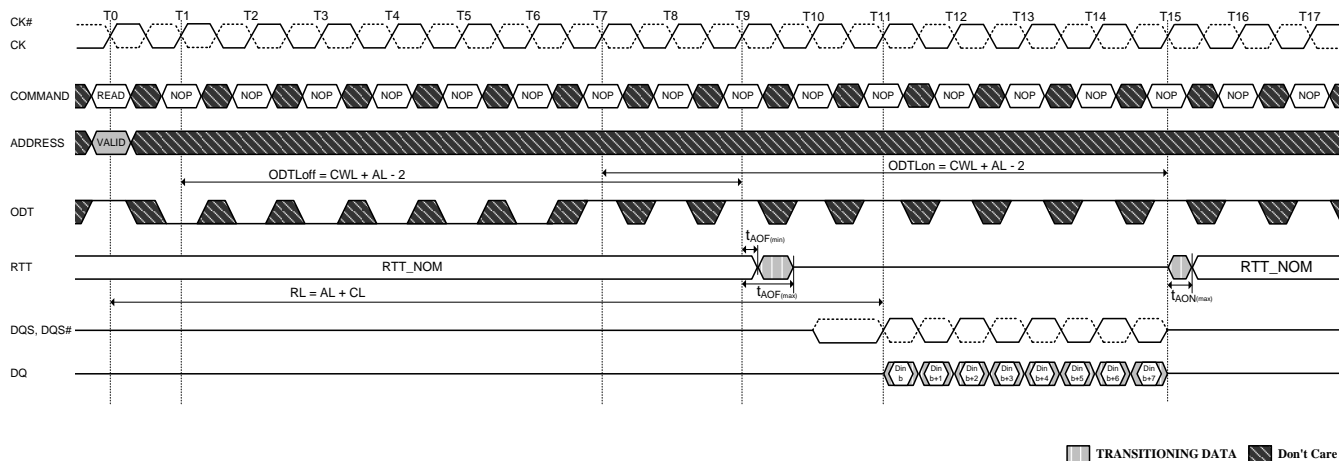
Figure 22. ODT must be disabled externally during Reads by driving ODT low ( CL=6 ; AL=CL-1=5 ; RL=AL+CL=11 ; CWL=5 ; ODTLon=CWL+AL-2=8 ; ODTLoff=CWL+AL-2=8 )
