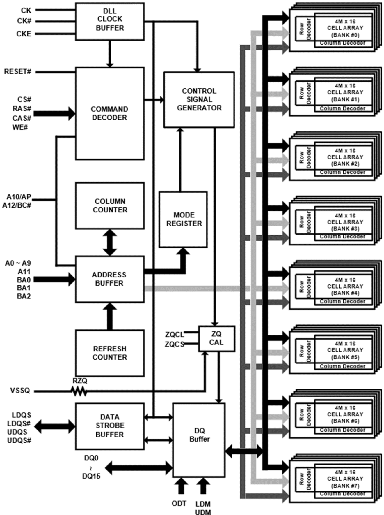
Figure 2. Block Diagram
