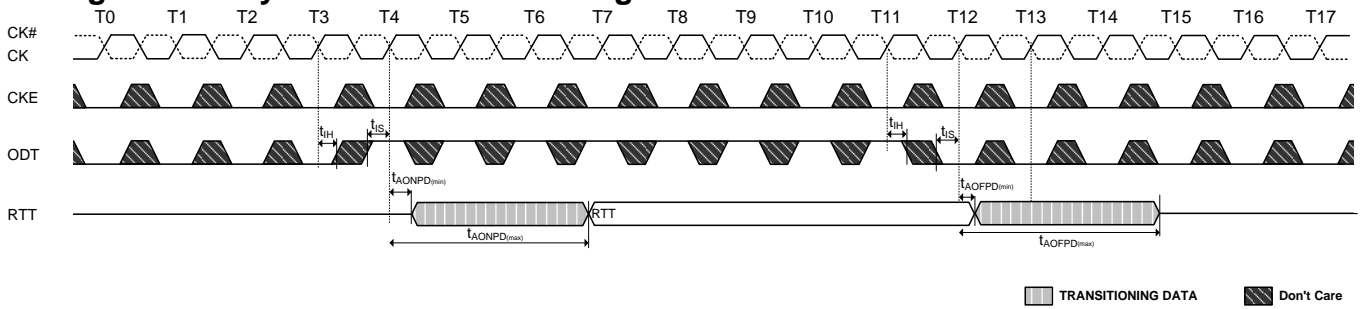
Figure 74. Asynchronous ODT Timings on DDR3/3L SDRAM with fast ODT transition
