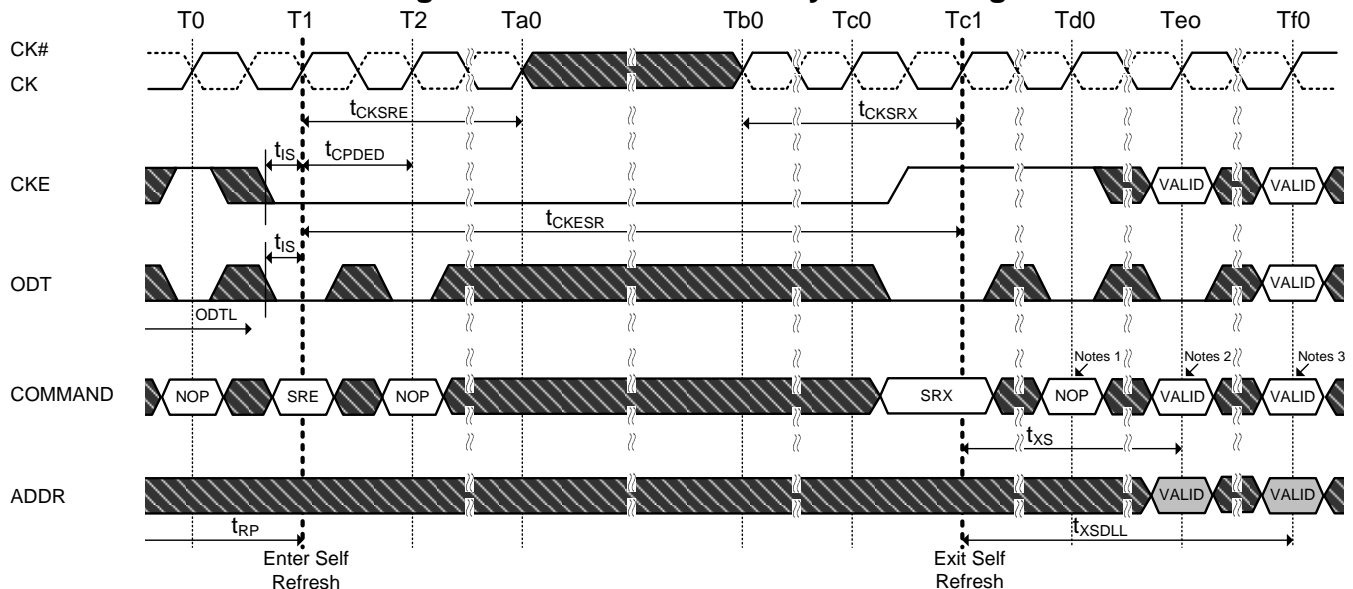
Figure 56. Self-Refresh Entry/Exit Timing
