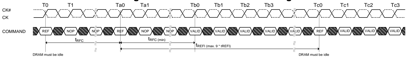
Figure 55. Refresh Command Timing
