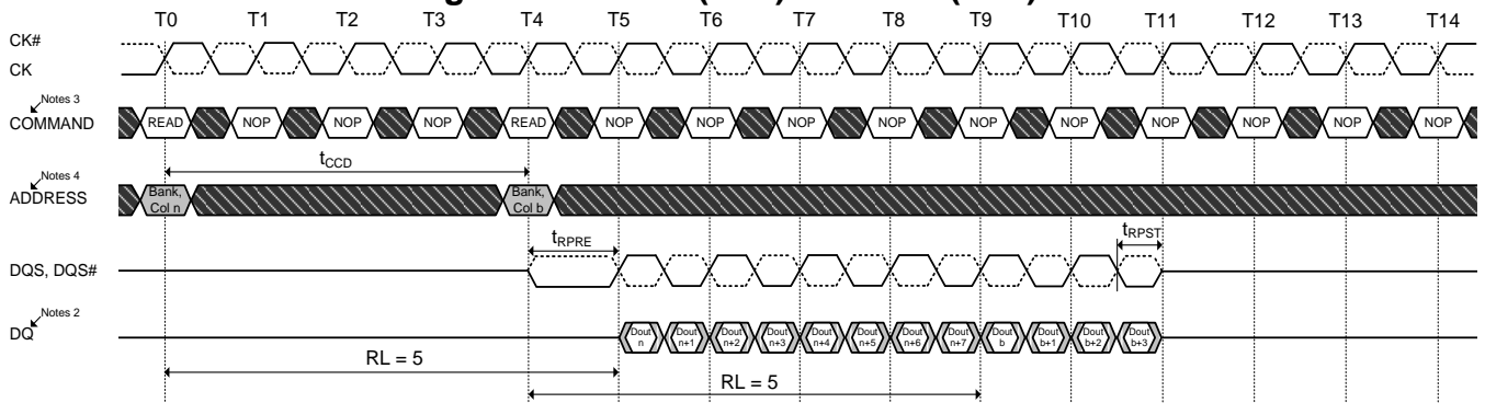
Figure 36. READ (BL8) to READ (BL4) OTF
