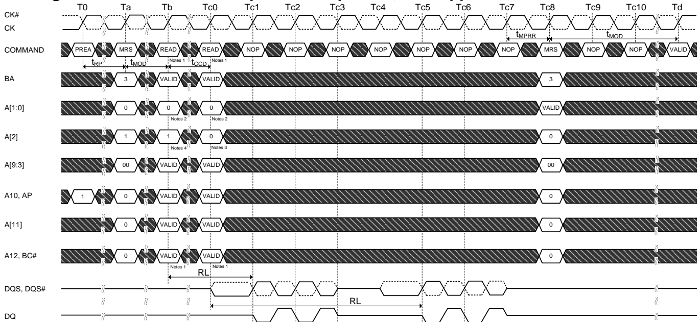
Figure 30. MPR Readout of predefined pattern, BC4 upper nibble then lower nibble
