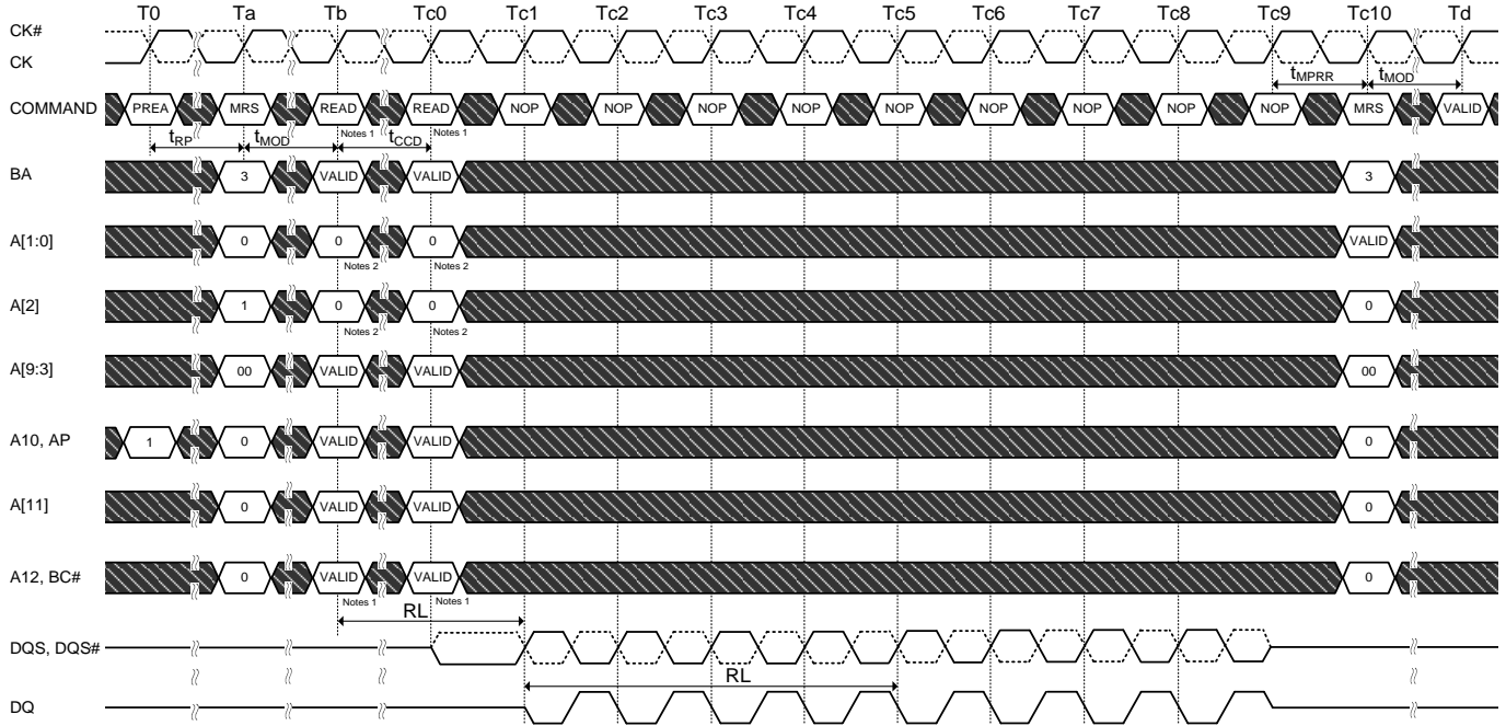
Figure 28. MPR Readout of predefined pattern, BL8 fixed burst order, back to back radout
