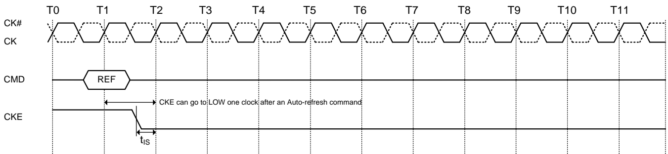
Figure 55. Refresh command to power-down entry
