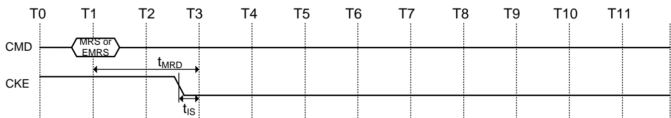
Figure 58. MRS/EMRS command to power-down entry
