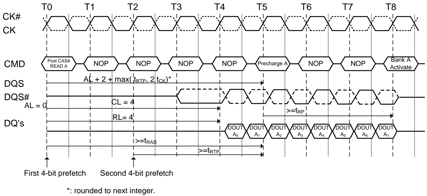
Figure 37. Burst read operation followed by precharge: (RL=4, AL=0, CL=4, BL=8, t_{RTP} > 2 clocks)
