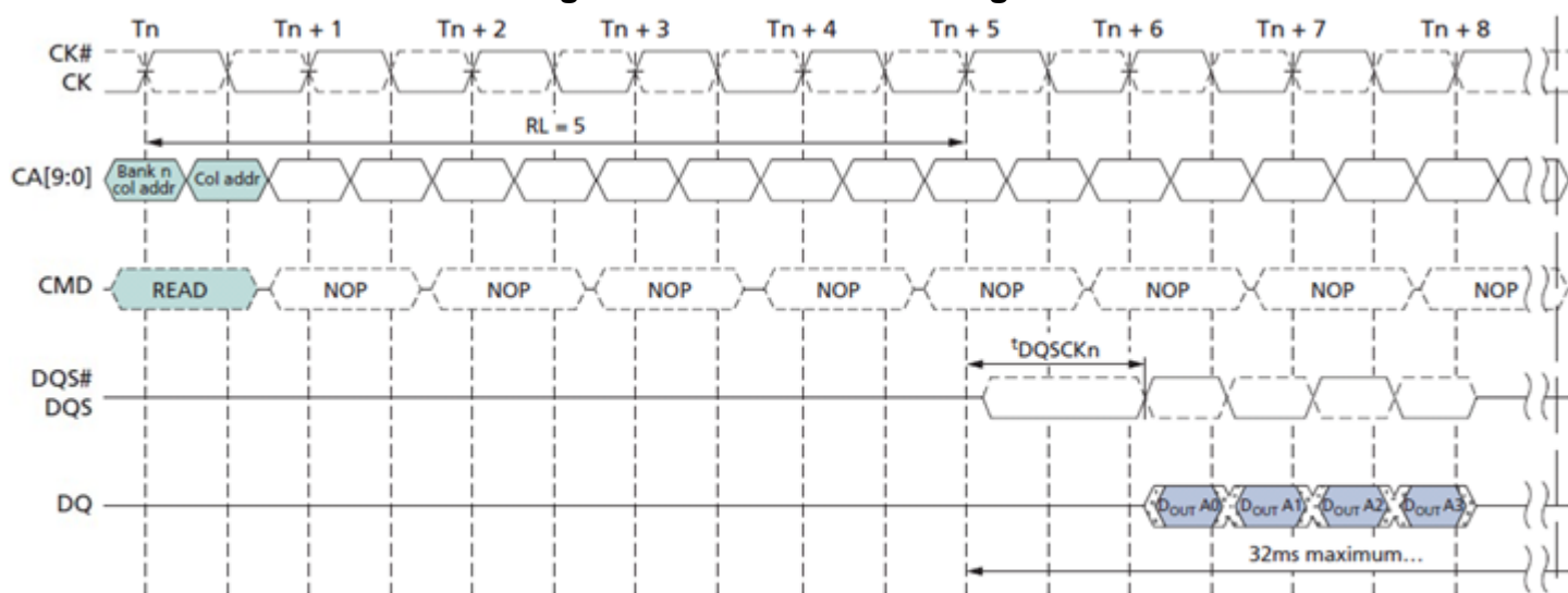
Figure 10. tDQSKDL Timing
