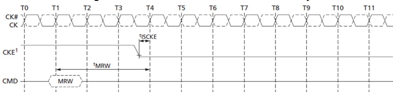
Figure 56. MRW Command to Power-Down Entry
