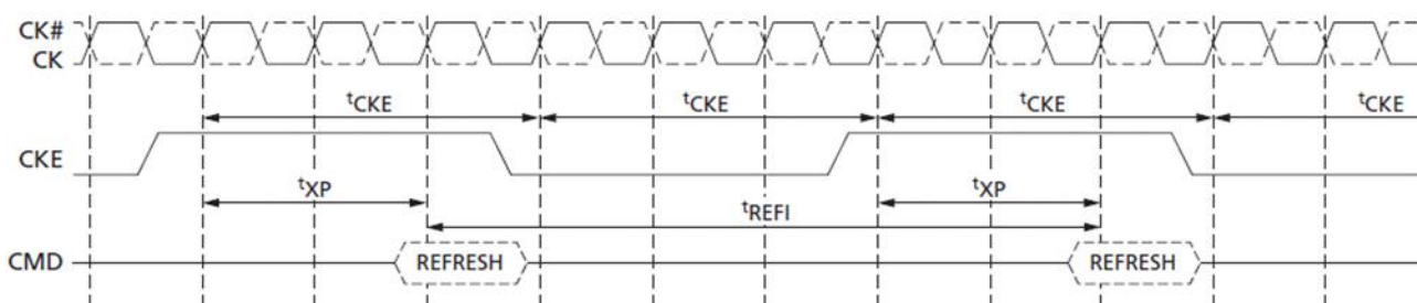
Figure 47. REFRESH-to-REFRESH Timing in CKE Intensive Environments
