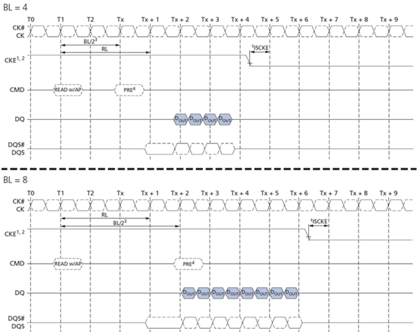
Figure 49. READ with Auto Precharge to Power-Down Entry
