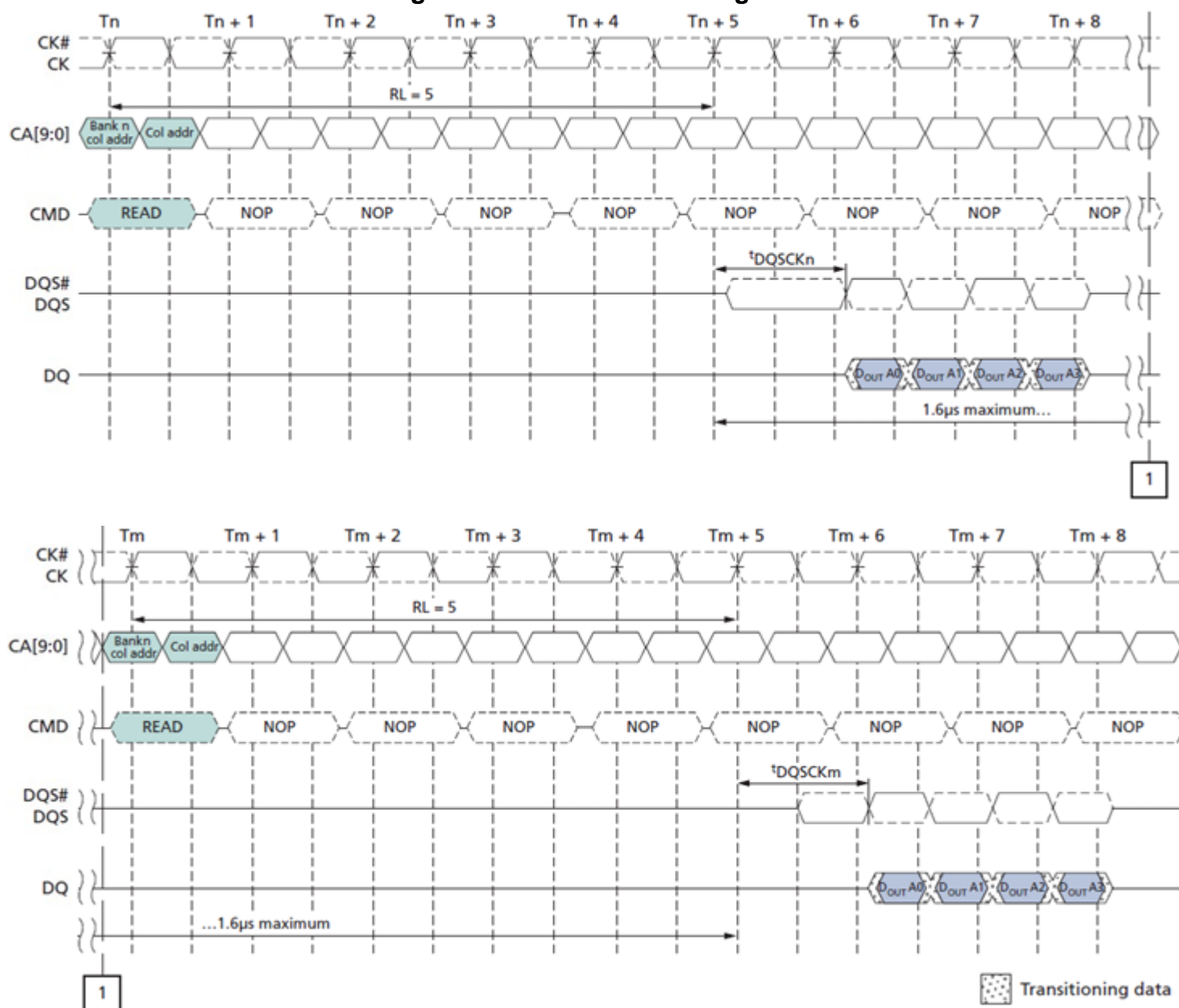
Figure 11. tDQSKDM Timing
