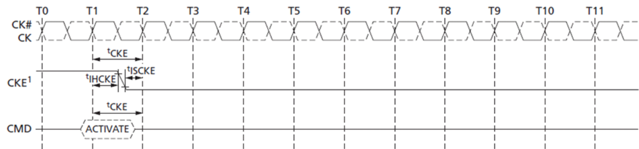
Figure 53. ACTIVATE Command to Power-Down Entry
