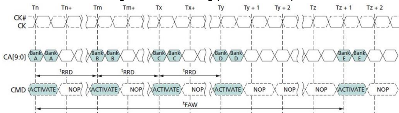
Figure 5. tFAW Timing (8-Bank Devices)
