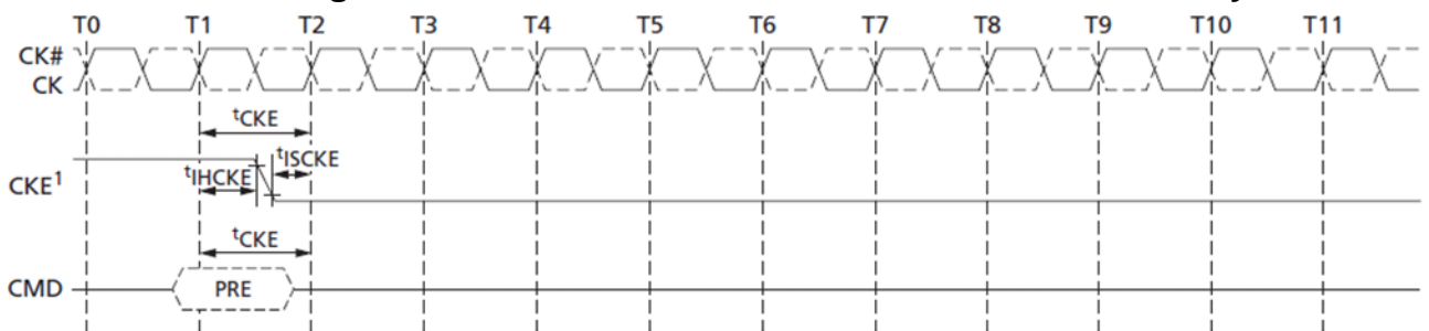
Figure 54. PRECHARGE Command to Power-Down Entry
