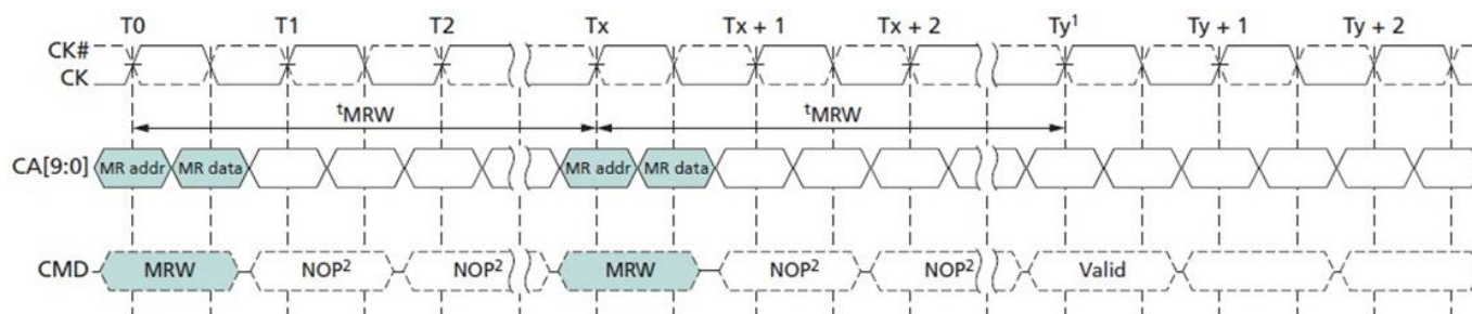
Figure 43. MODE REGISTER WRITE Timing – RL = 3, tMRW = 5
