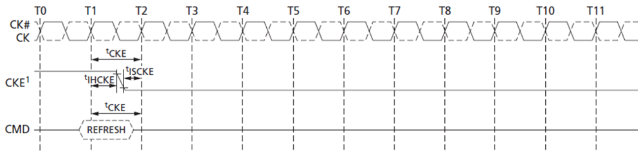
Figure 52. REFRESH Command to Power-Down Entry
