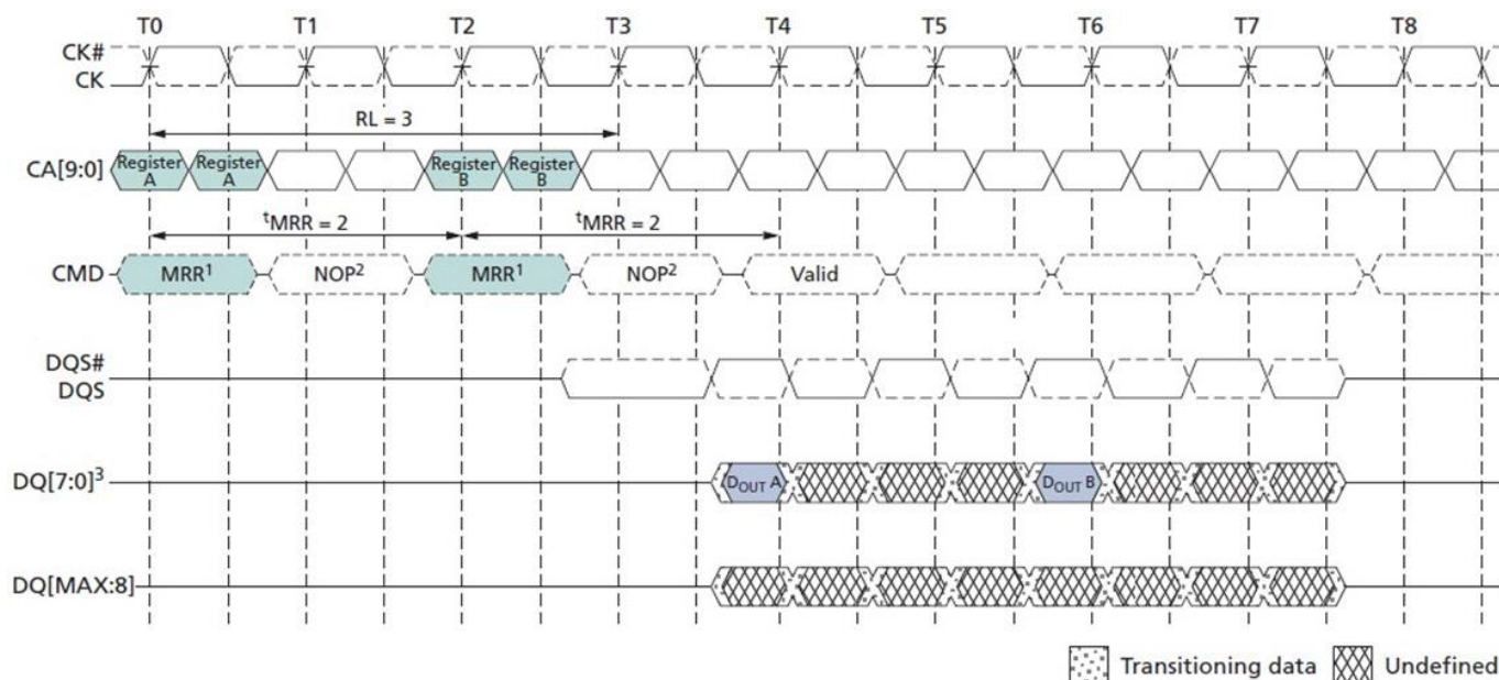
Figure 38. MRR Timing – RL = 3, tMRR = 2
