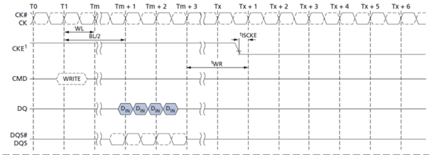
Figure 50. WRITE to Power-Down Entry
