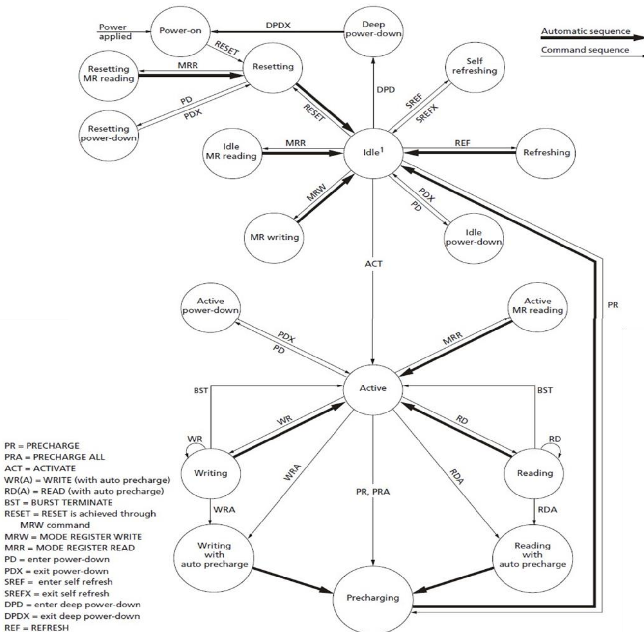
Figure 2. Simplified Bus Interface State Diagram
