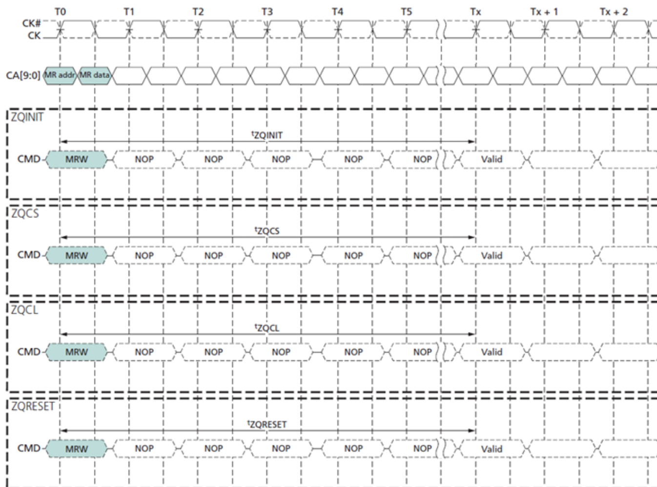
Figure 44. ZQ Timings
