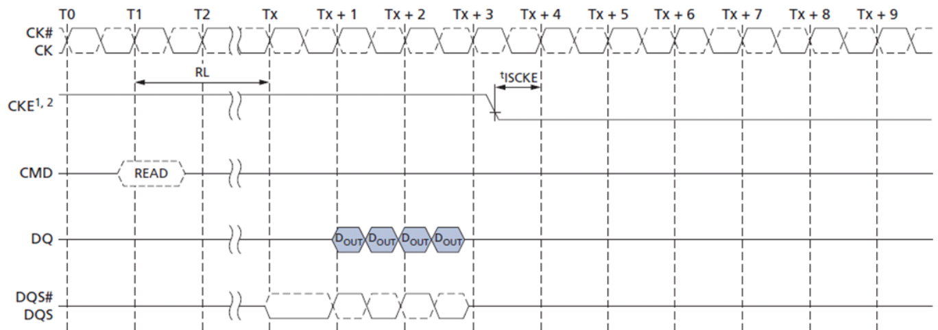
Figure 48. READ to Power-Down Entry
