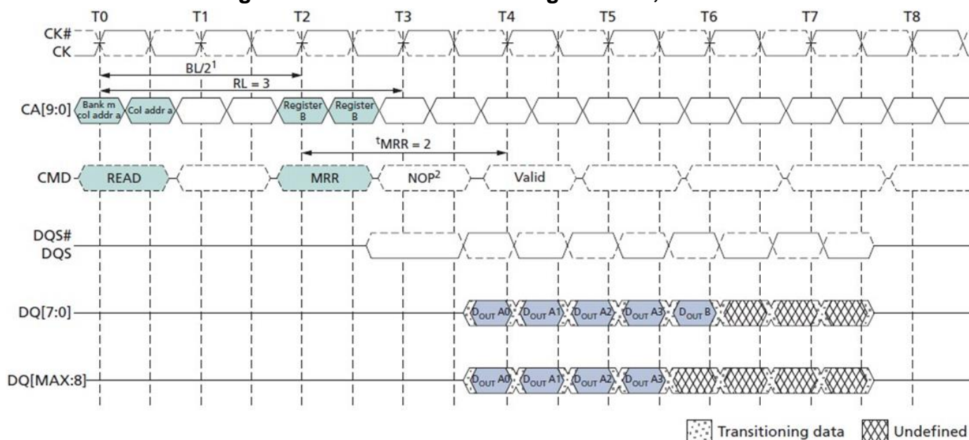
Figure 39. READ to MRR Timing – RL = 3, tMRR = 2
