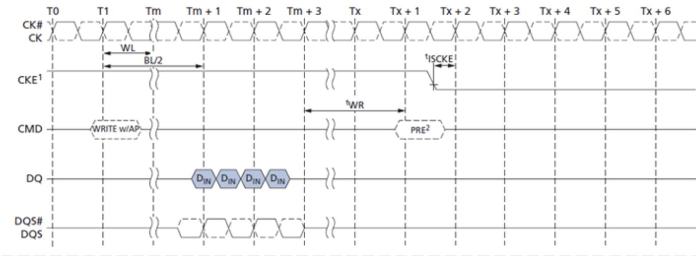
Figure 51. WRITE with Auto Precharge to Power-Down Entry
