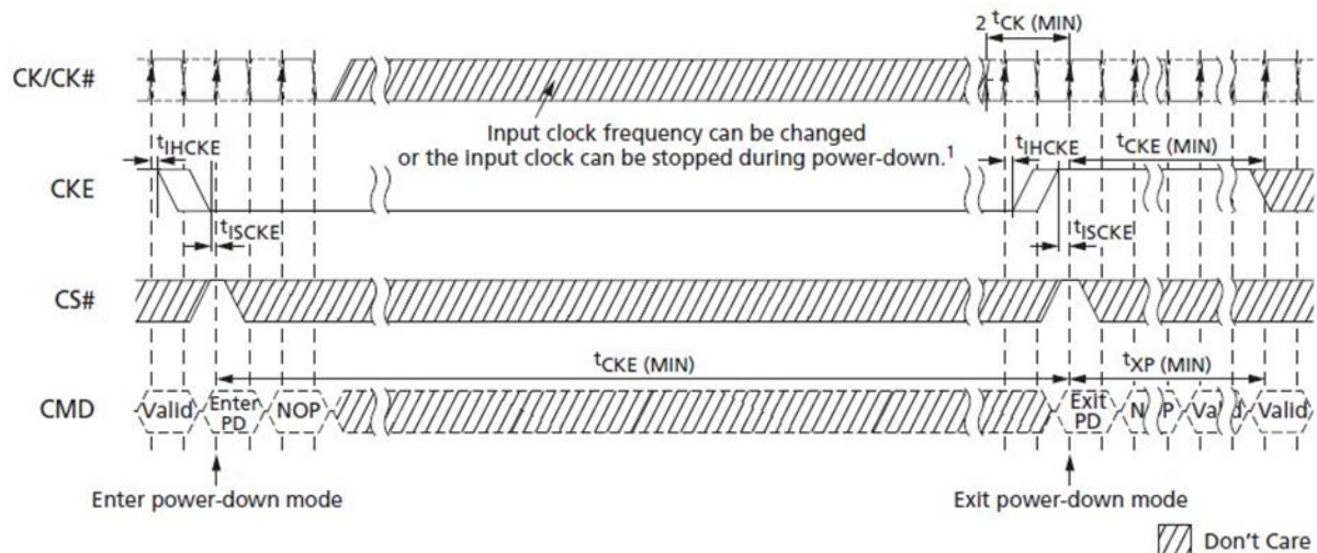
Figure 45. Power-Down Entry and Exit Timing
