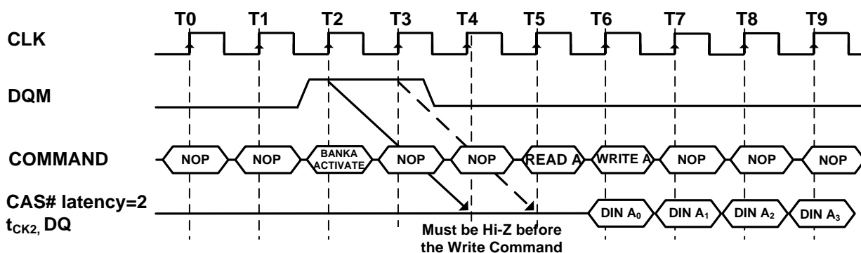
Figure 6. Read to Write Interval (Burst Length ≥ 4, CAS# Latency = 2)
